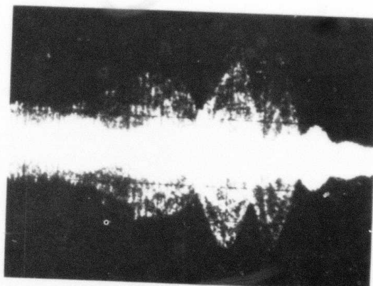
d. A 1\text{-}\mu\text{m} thick film of aluminum on silicon, f = 1100 MHz.
