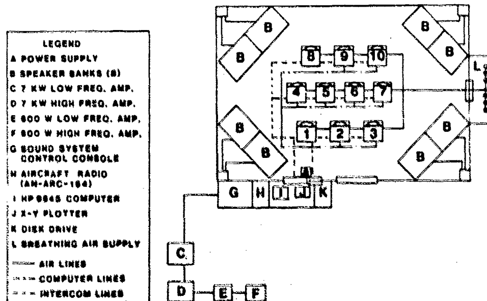
Figure 1. SUBSYSTEMS INTEGRATION
