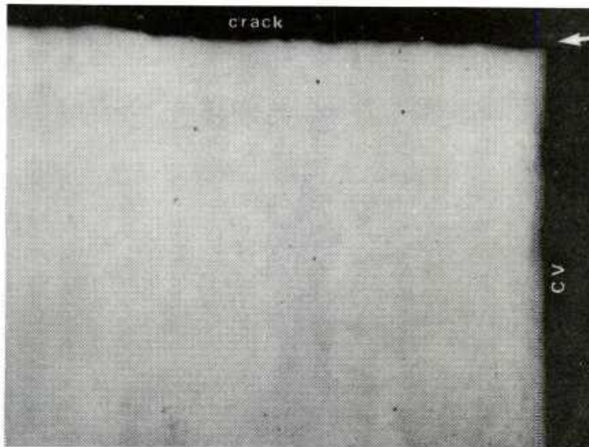
Figure 61. Polished Section Through the Fatigue Origin (arrow) Shown in Figures 59 and 60. Magnification: 200X
