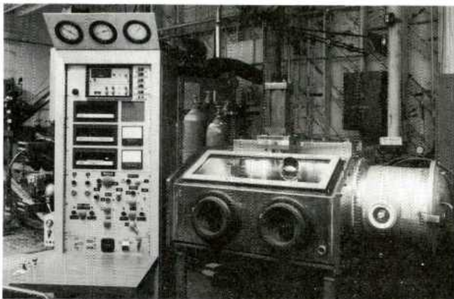
Figure 50. Hot Coining Press and Control Panel (#80-1286)
