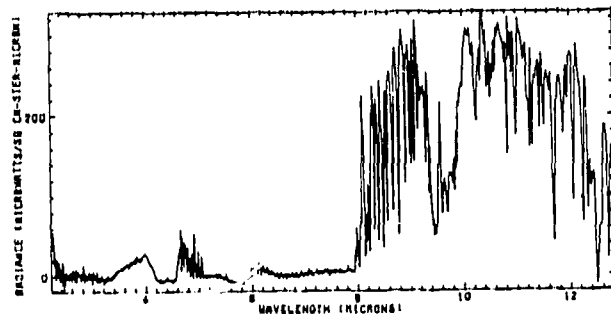
C. Trees/Sky Difference Spectrum
