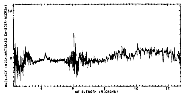
C. Sand/Surf Difference Spectrum
