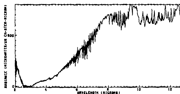
B. Radiance Spectrum of Sky
