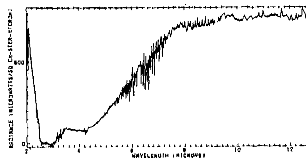
B. Radiance Spectrum of Surf
