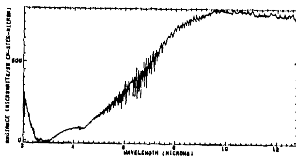
A. Radiance Spectrum of Mountain
