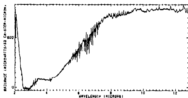
A. Radiance Spectrum of Sand
