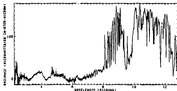
C. Rock/Water Difference Spectrum
