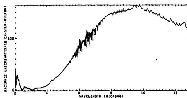
A. Radiance Spectrum of Trees
