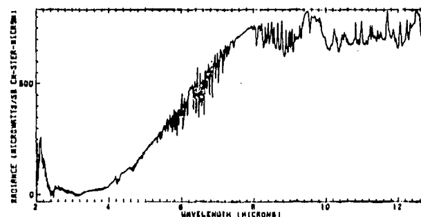
B. Radiance Spectrum of Water
