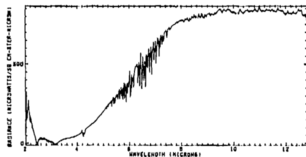
A. Radiance Spectrum of Rock
