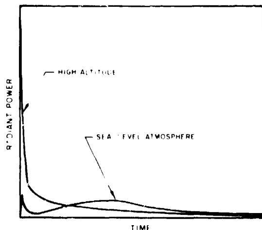
Figure 2.133. Qualitative comparison of rates of arrival of thermal radiation at a given distance from high-altitude and sea-level bursts.
