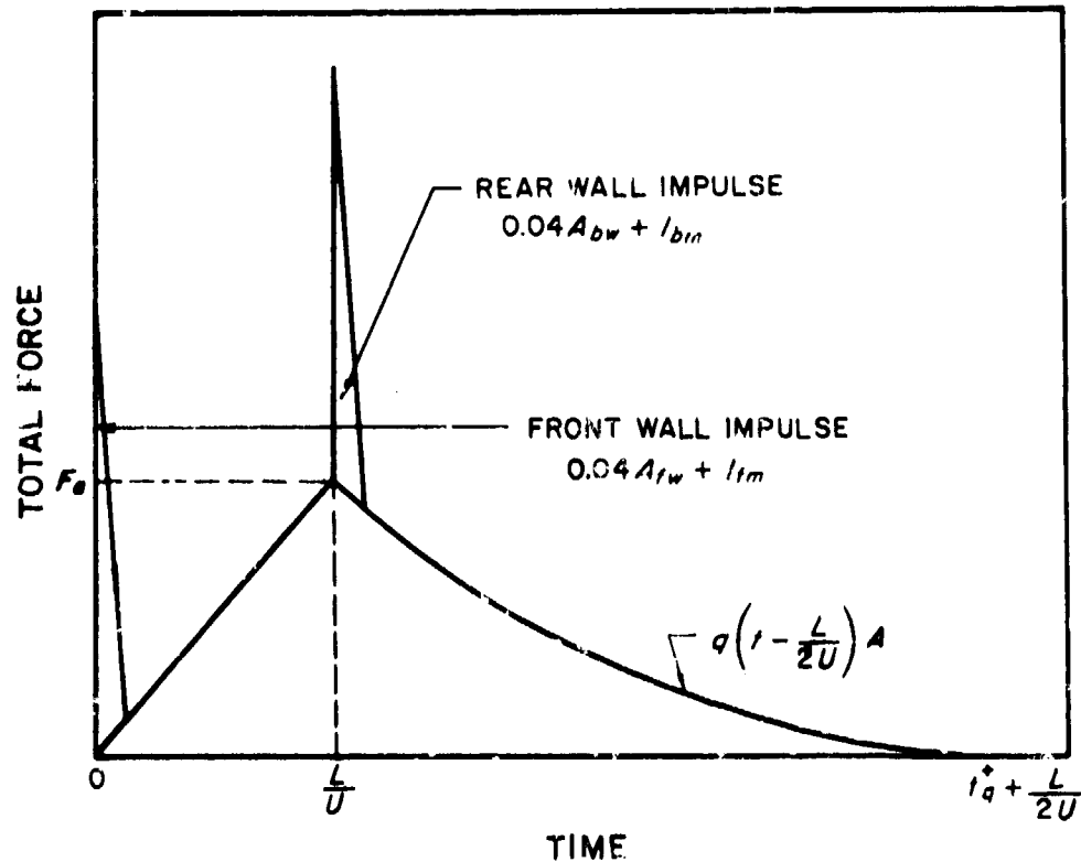
Figure 4.56. Net horizontal loading of an open frame structure.
