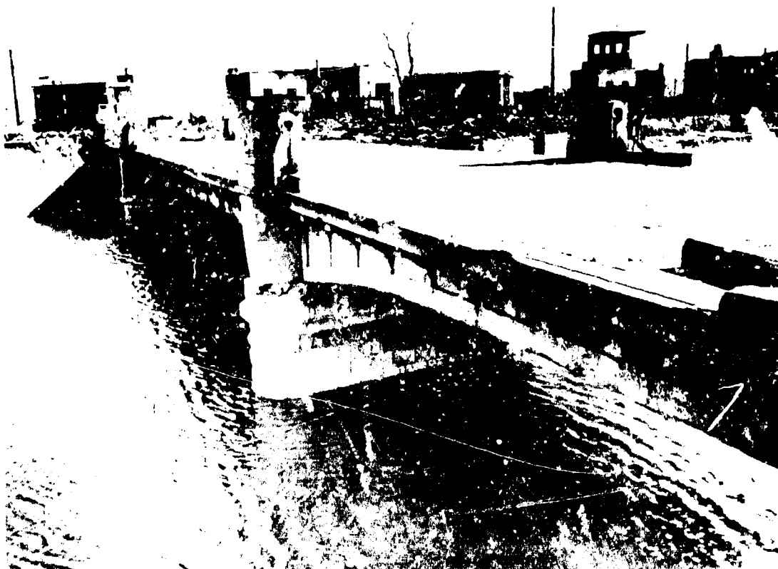
Figure 5.127a. Bridge with deck of reinforced concrete on steel-plate girders; outer girder had concrete facing (270 feet from ground zero at Hiroshima). The railing was blown down but the deck received little damage so that traffic continued.
