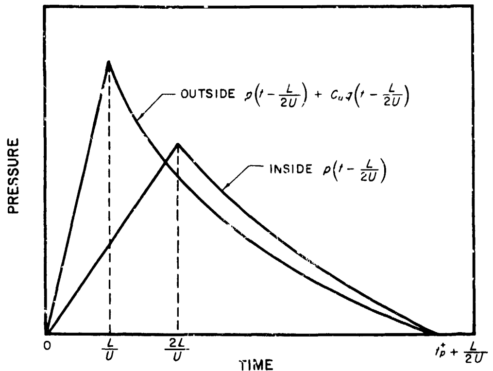
Figure 4.49 Average side and top loading of partially open box-like structure.
