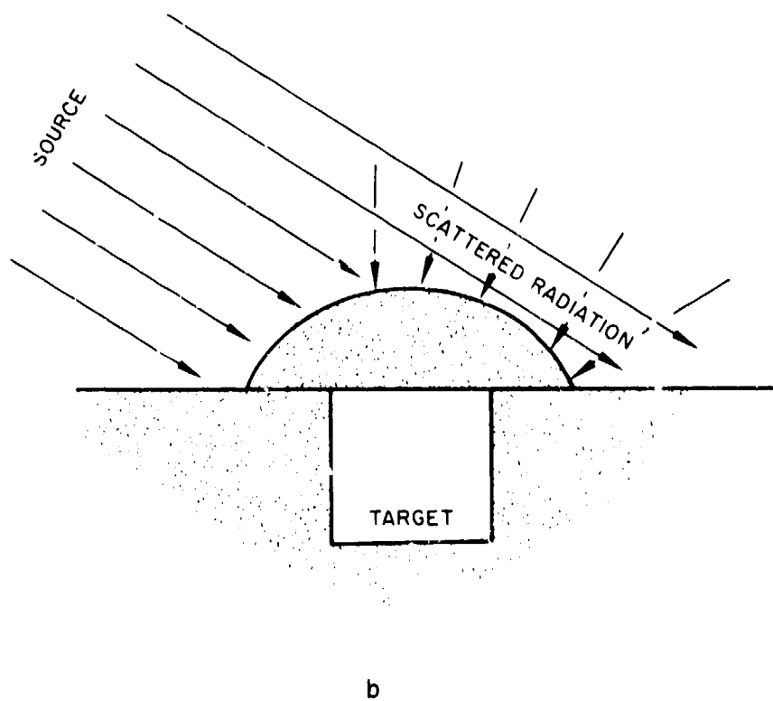
Figure 8.45b. Target shielded from scattered gamma radiation.
