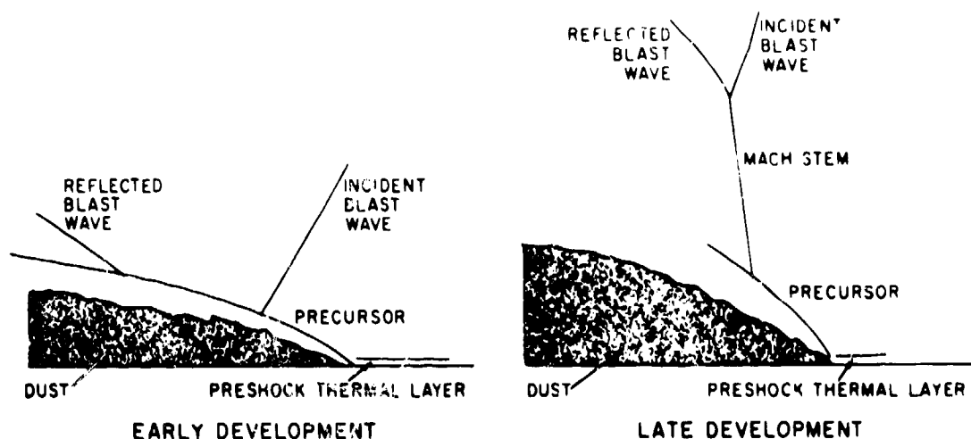
Figure 3.81. Precursor characteristics.
