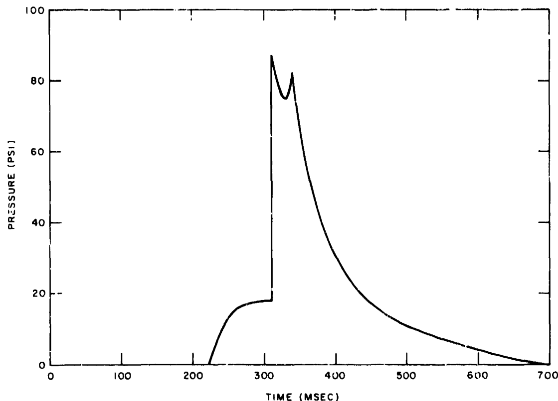
Figure 4.67a. Nonideal incident air blast (shock) wave.
