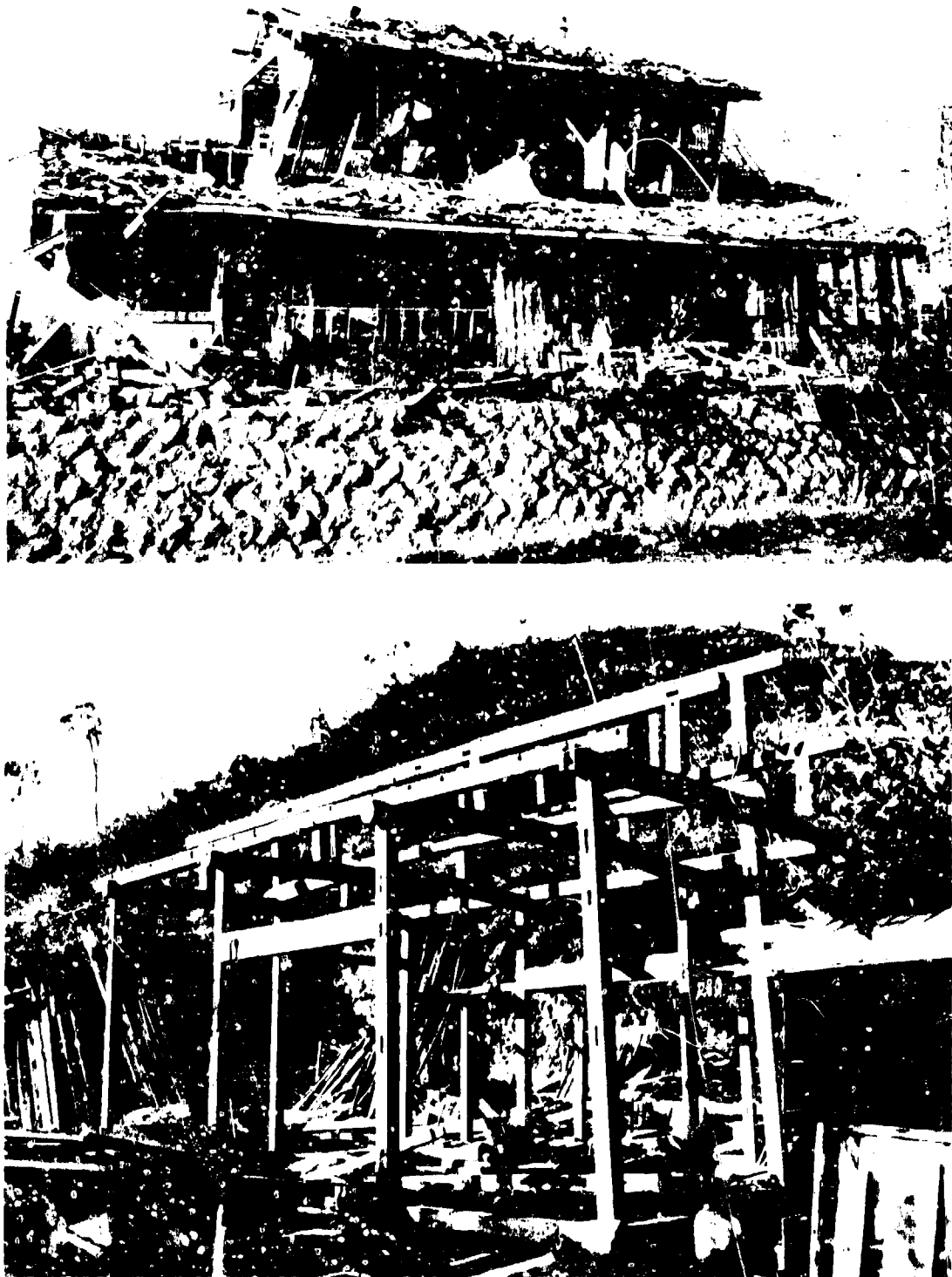
Figure 5.52. Upper photo; Wood-frame building; 1.0 mile from ground zero at Hiroshima. Lower photo: Frame of residence under construction, showing small tenons.
