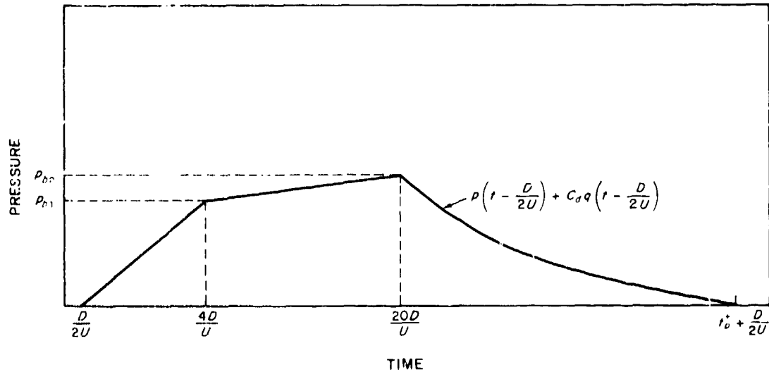
Figure 4.60. Average pressure variation on the back face of a cylinder.
