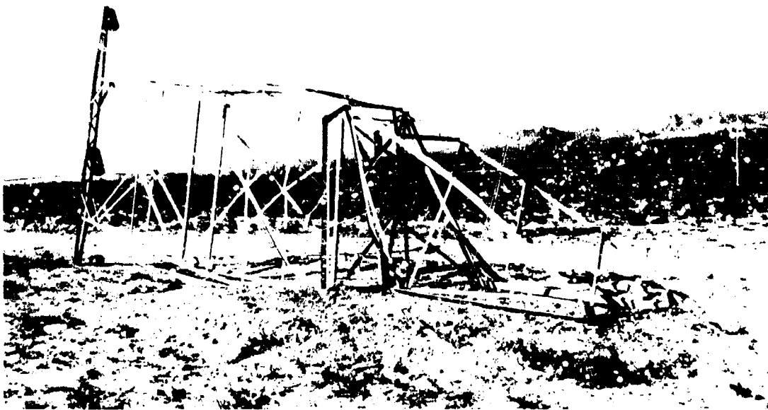
Figure 5.102a. Collapsed suspension tower (5 psi peak overpressure, 0.7 psi dynamic pressure from 30-kiloton explosion), Nevada Test Site.
