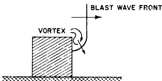
Figure 4.27. Blast wave moving down rear of cube.
