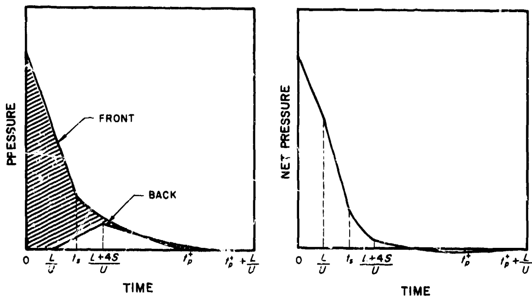
Figure 4.45. Net horizontal loading of closed box-like structure.
