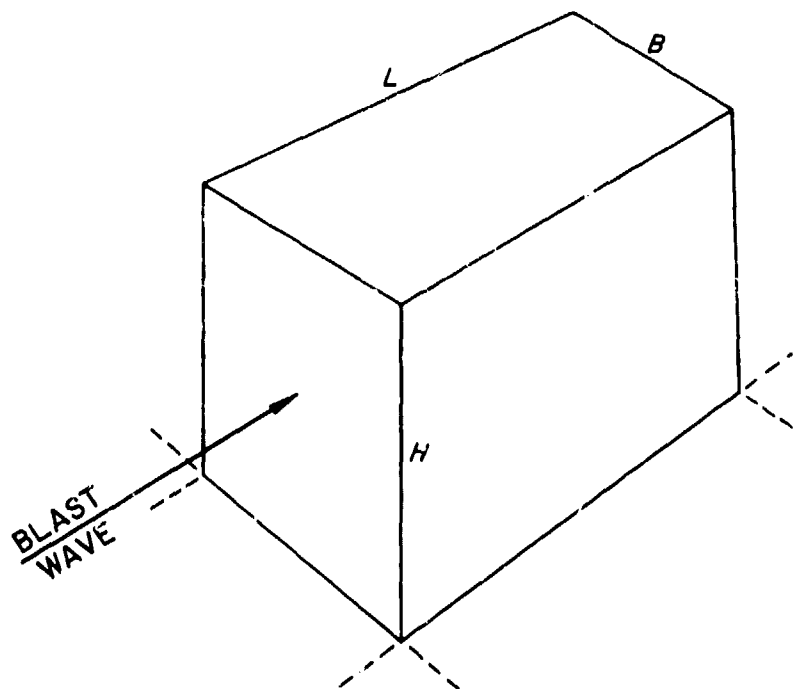
Figure 4.41. Representation of closed box-like structure.
