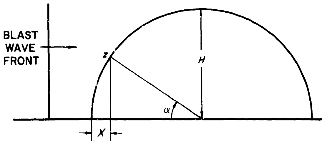
Figure 4.62. Representation of a typical semicircular arched structure.
