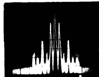
1 kHz Bandwidth, 20 kHz/div.. 5 sec/div.
