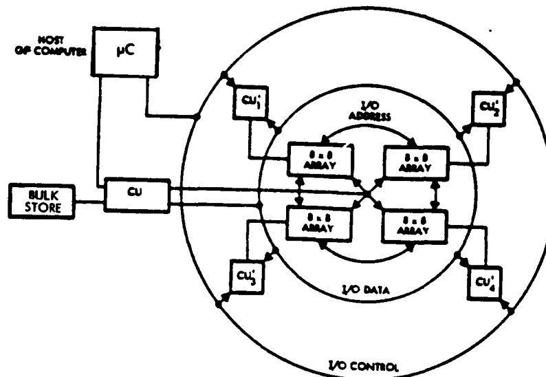
Figure 4-10 - Array Processor System - Multiple External Array
