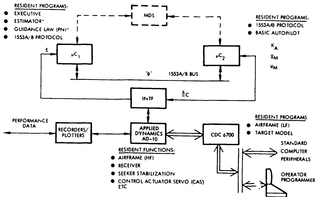
Figure 3-16 Navy/Raytheon Hardware-in-the-Loop Federated \mu C System for Missile Performance Simulation
