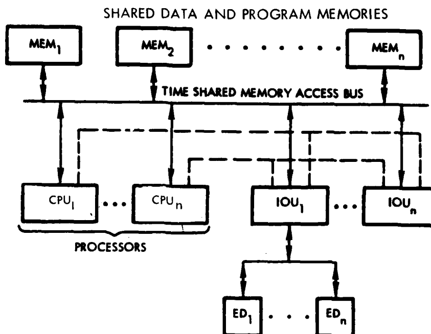
Figure 4-1 - Multiprocessor System - Single Time-Shared Memory Access Bus
