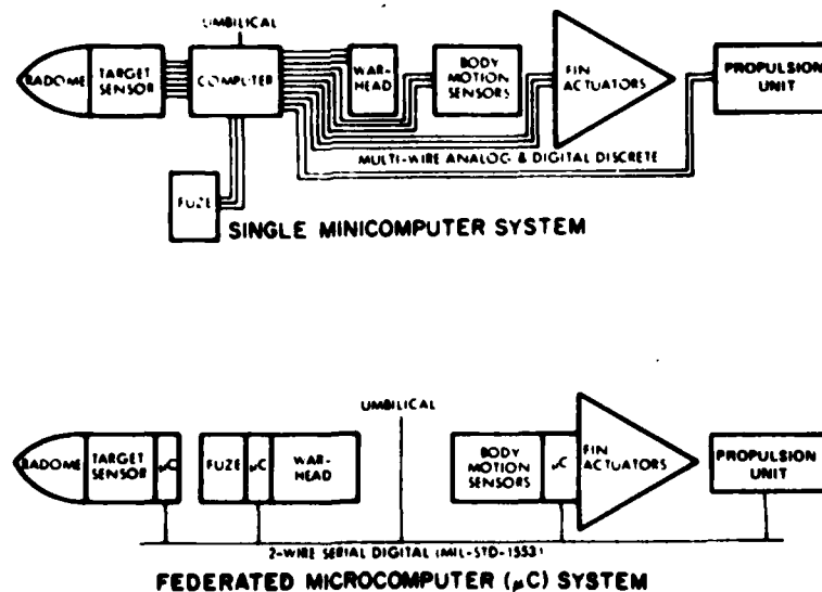
Figure 3-1 - Single versus Federated Missile Guidance and Control Systems
