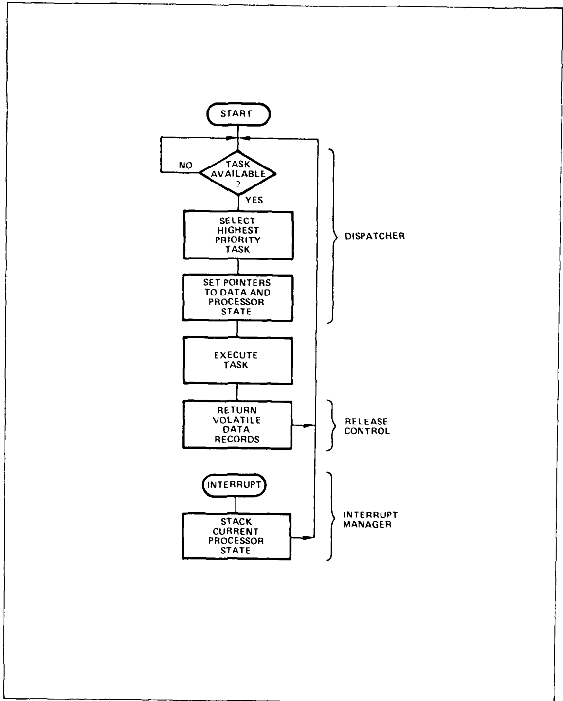
Figure 6-8 - Floating Executive (Multiprogrammed)
