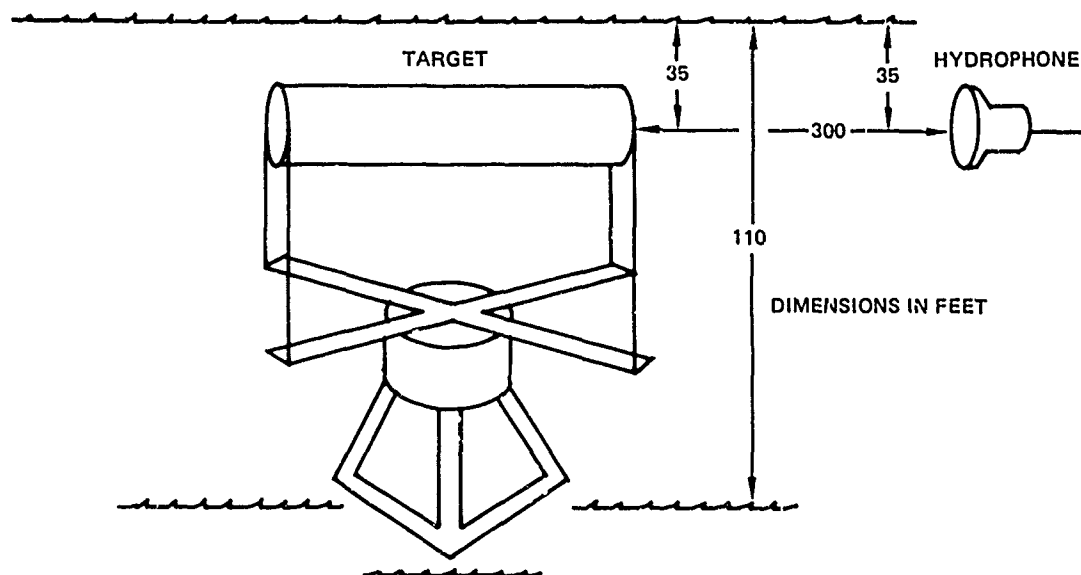
Figure 1. Target rotator.
