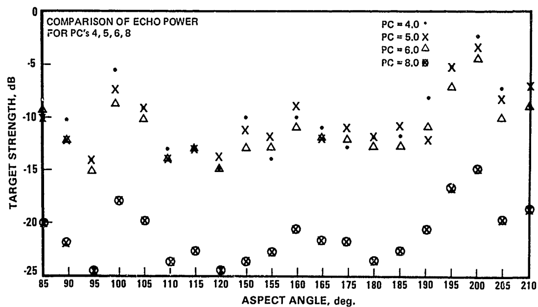
Figure 27. Comparison of Echo Power for PC's 4, 5, 6, 8.
