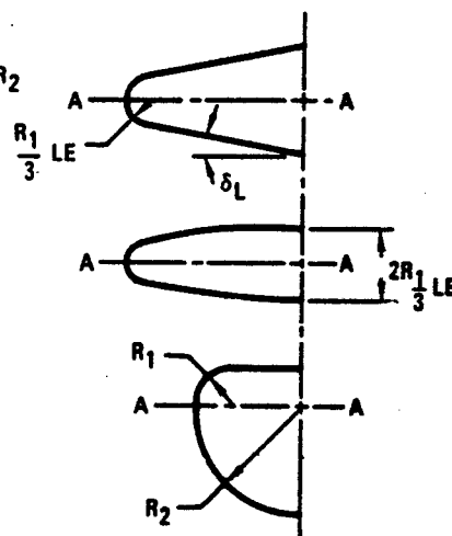
FIGURE 20 INPUT FOR NAMLIST LARWB - LOW ASPECT RATIO WING, WING-BODY INPUT
