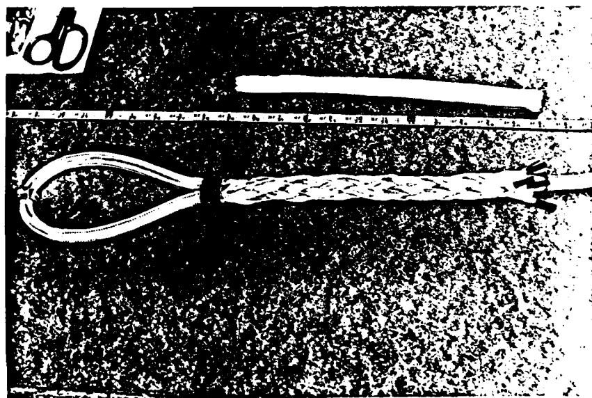
FIGURE 19. TUCKING COMPLETED
