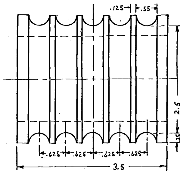
Five-Groove Spool
