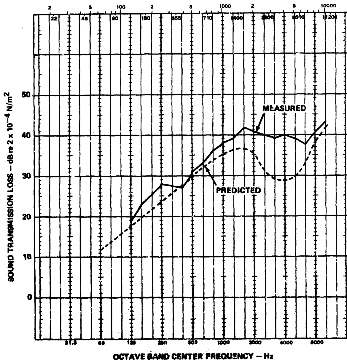
Figure 65. Crew compartment enclosure - sound transmission loss, 1/2-inch plexiglass.
