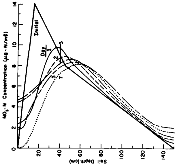
Figure 6. Simulated \text{NO}_3\text{-N} distributions for one week following wastewater application and for \bar{k}_1 = 0.1 \text{ h}^{-1} , K_D = 0.25 \text{ cm}^3/\text{g} and I_{\text{max}} = 0.001 \text{ µg N/h cm} .
