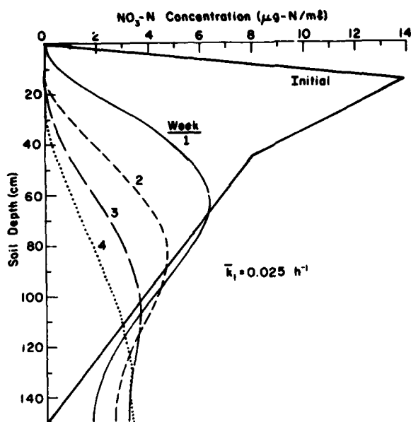
Figure 8. Simulated concentration distributions of \text{NO}_3\text{-N} in the soil profile where weekly application of 5 cm of wastewater was maintained. Model parameters were \bar{k}_1 = 0.025 \text{ h}^{-1} , K_D = 0.25 \text{ cm}^3/\text{g} and I_{\text{max}} = 0.001 \text{ } \mu\text{g N/h cm} .
