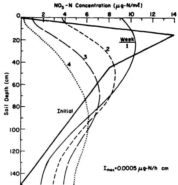
Figure 17. Simulated concentration distribution of \text{NO}_3\text{-N} in the soil profile where \bar{k}_1 = 0.1 \text{ h}^{-1} , K_D = 0.25 \text{ cm}^3/\text{g} and I_{\text{max}} = 0.0005 \text{ } \mu\text{g N/h cm} .
