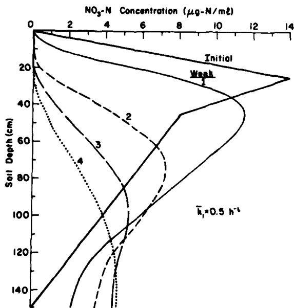
Figure 12. Simulated concentration distributions of \text{NO}_3\text{-N} in the soil profile where weekly application of 5 cm of wastewater was maintained. Model parameters were \bar{k}_1 = 0.5 \text{ h}^{-1} , K_D = 0.05 \text{ cm}^3/\text{g} and l_{\text{max}} = 0.001 \text{ } \mu\text{g N/h cm} .
