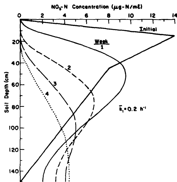
Figure 11. Simulated concentration distributions of \text{NO}_3\text{-N} in the soil profile where weekly application of 5 cm of wastewater was maintained. Model parameters were \bar{k}_1 = 0.2 \text{ h}^{-1} , K_D = 0.25 \text{ cm}^3/\text{g} and l_{\text{max}} = 0.001 \text{ } \mu\text{g N/h cm} .
