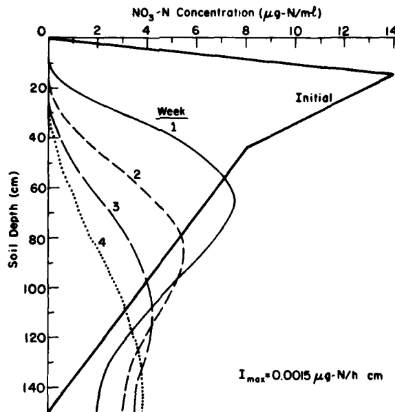
Figure 18. Simulated concentration distribution of \text{NO}_3\text{-N} in the soil profile where \bar{k}_1 = 0.1 \text{ h}^{-1} , K_D = 0.25 \text{ cm}^3/\text{g} and I_{\text{max}} = 0.0015 \text{ } \mu\text{g N/h cm} .
