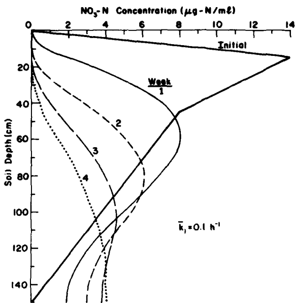
Figure 10. Simulated concentration distributions of \text{NO}_3\text{-N} in the soil profile where weekly application of 5 cm of wastewater was maintained. Model parameters were \bar{k}_1 = 0.1 \text{ h}^{-1} , K_D = 0.25 \text{ cm}^3/\text{g} and l_{\text{max}} = 0.001 \text{ } \mu\text{g N/h cm} .
