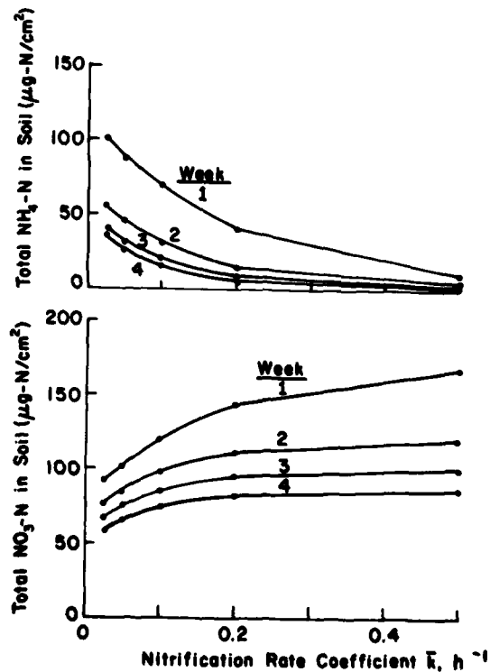
Figure 13. Nitrification rate coefficient \bar{k}_1 vs total \text{NH}_4\text{-N} and \text{NO}_3\text{-N} in the soil profile.
