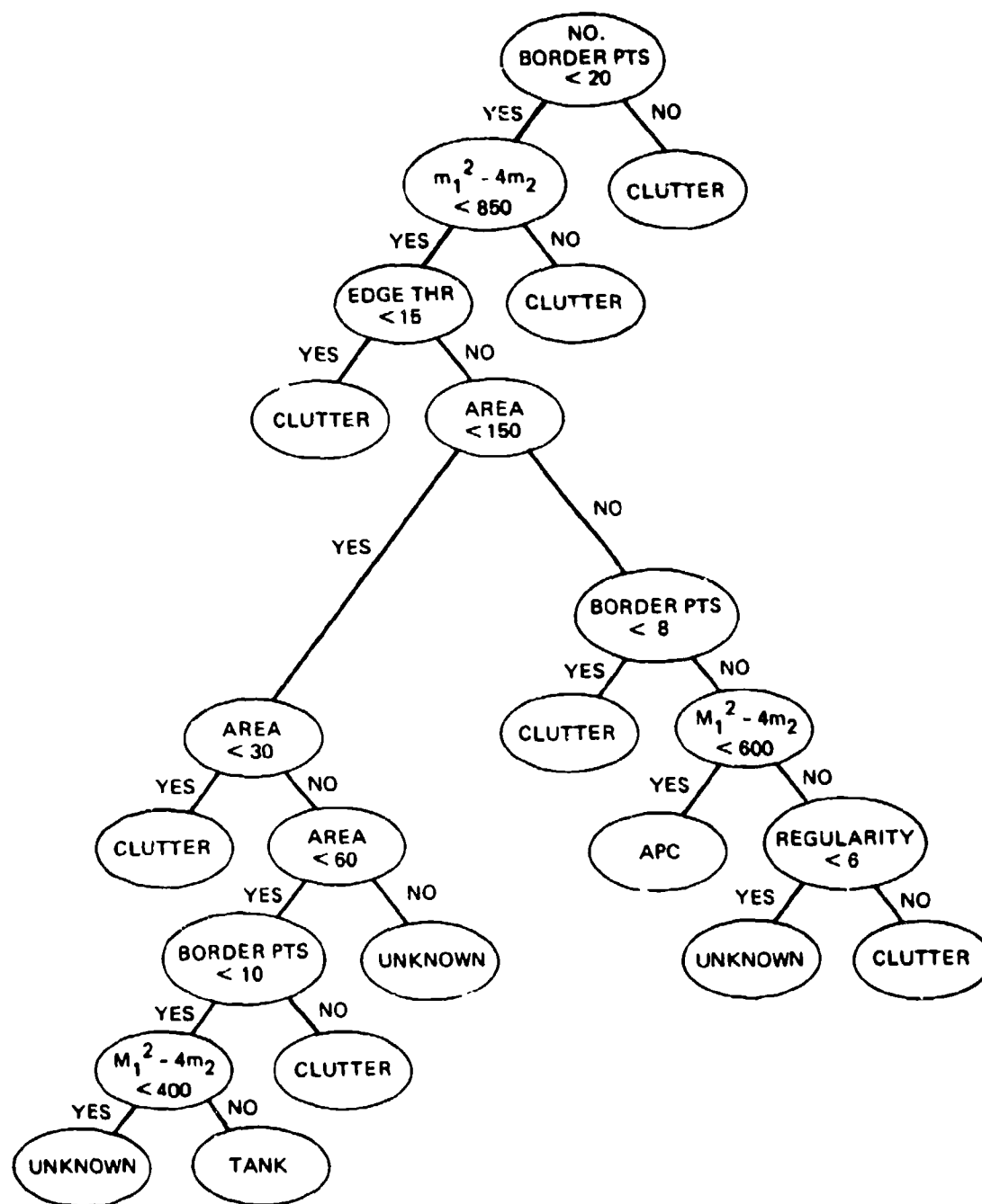
Figure 4-7. A numerical decision tree to classify an APC or tank based on auto-cuer segmentation features.
