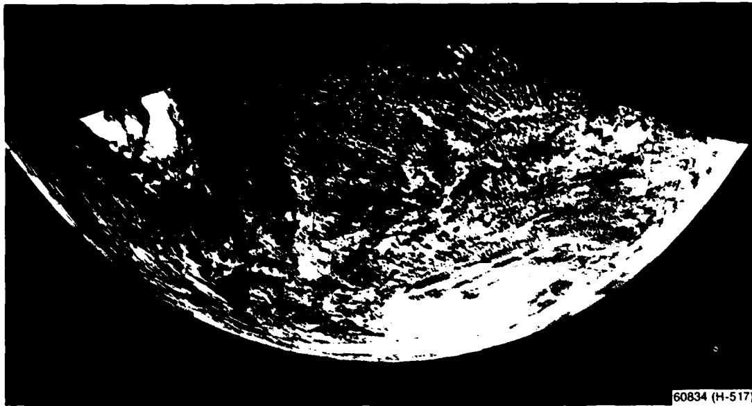
FIRST HIGH-ALTITUDE PICTURE OF A HURRICANE IN A TROPICAL STORM (5 OCT. 1954)
