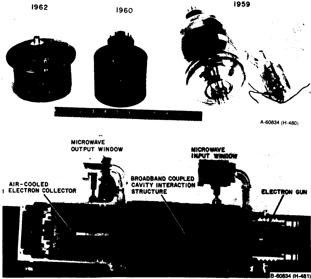
NOVEL DECEPTION PULSE REPEATER TUBES (1954)
