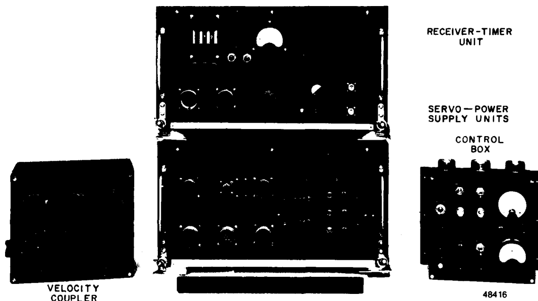
THE FIRST AIRCRAFT OMEGA RECEIVER - THE MARK I
