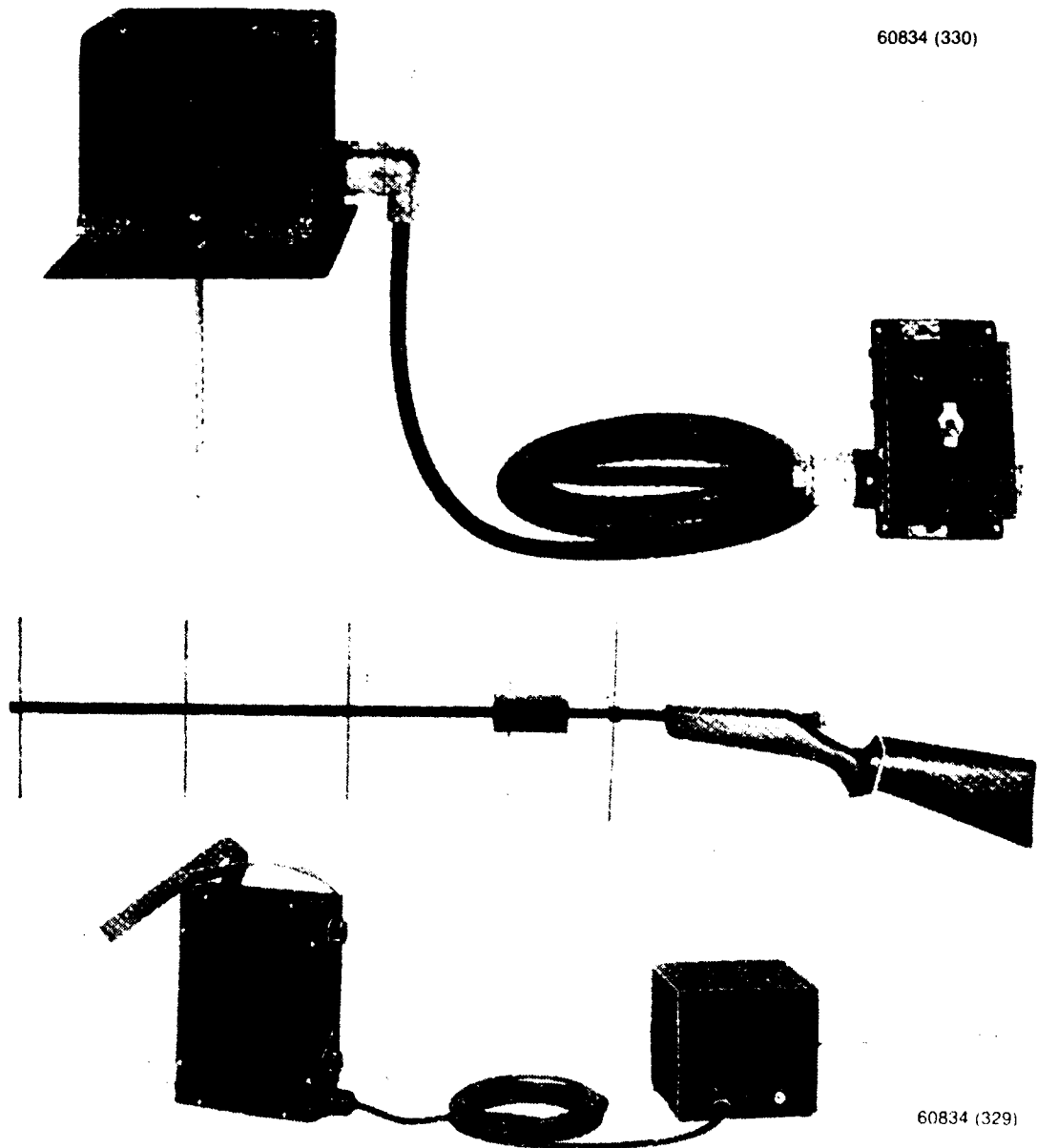
THE FIRST RADIO RECOGNITION IFF SYSTEM IN THE UNITED STATES THE MODEL XAE (1937)
