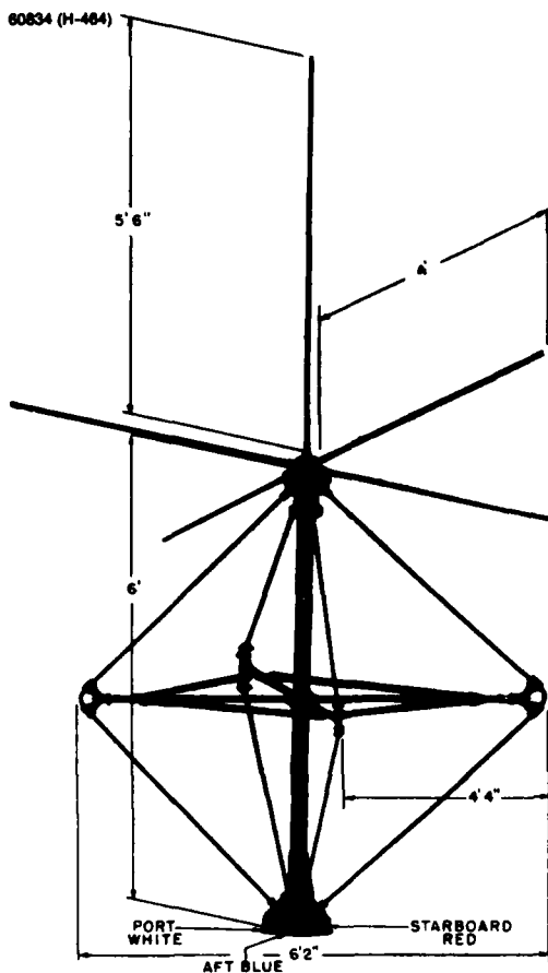
THE FIRST U.S. HIGH-FREQUENCY SHIP DIRECTION FINDER EMPLOYING FIXED CROSS-LOOP ANTENNAS, WITH BEARING DISPLAYED ON A CATHODE-RAY TUBE THROUGH THE USE OF A ROTATING GONIOMETER AND A SYNCHRONOUSLY ROTATING MAGNETIC DEFLECTION YOKE ABOUT THE TUBE (1943)
