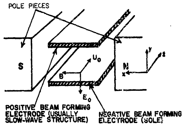
FIGURE 5 - CROSSED-FIELD TWT
