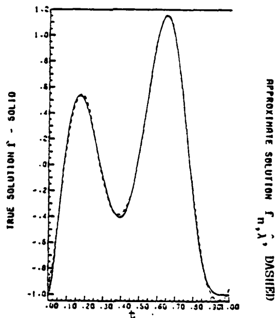
(c) The true and estimated second derivative.
