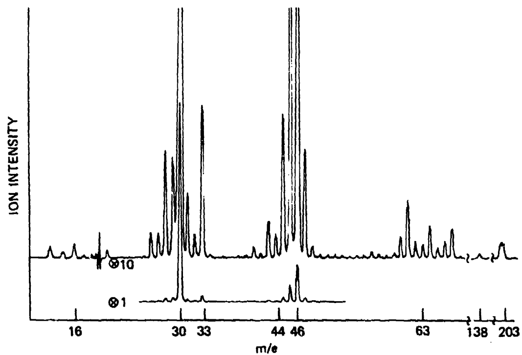
FIGURE 3 MASS SPECTRA OF DFF AND ITS PYROLYSIS PRODUCTS
