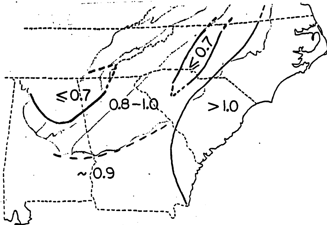
FIGURE 16. Characteristic Heat Flow Zones of Alabama, Georgia, South and North Carolina. Light lines indicate piedmont, Blue Ridge, and valley and ridge physiographic provinces. 30
