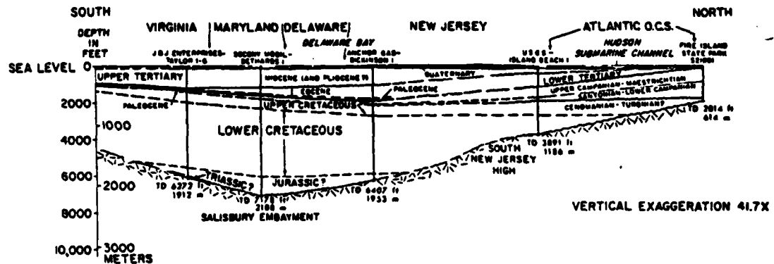
FIGURE 7. Cross Section Parallel to the Coastline Between the Delmarva Peninsula and Long Island. 8
