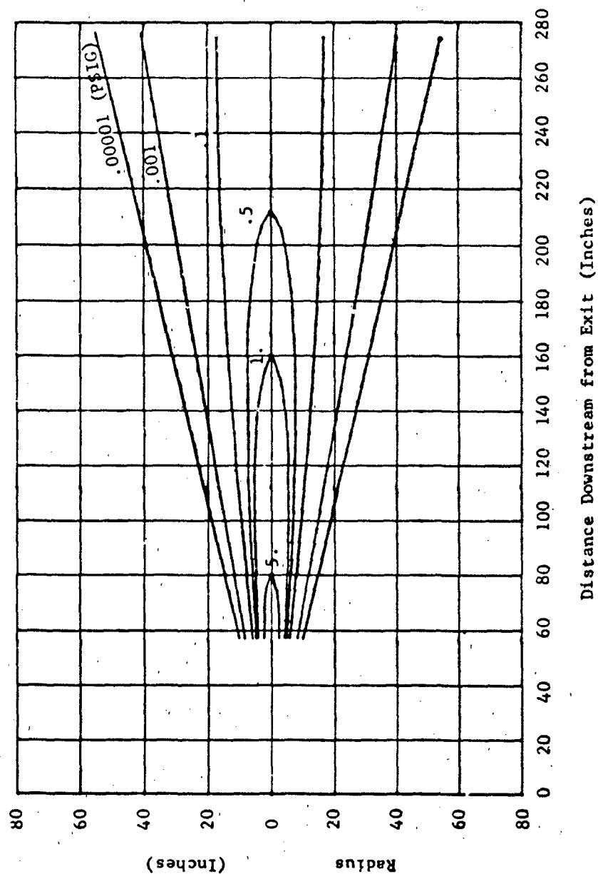
Figure 2-2. Pressure Plume Plot Region III
