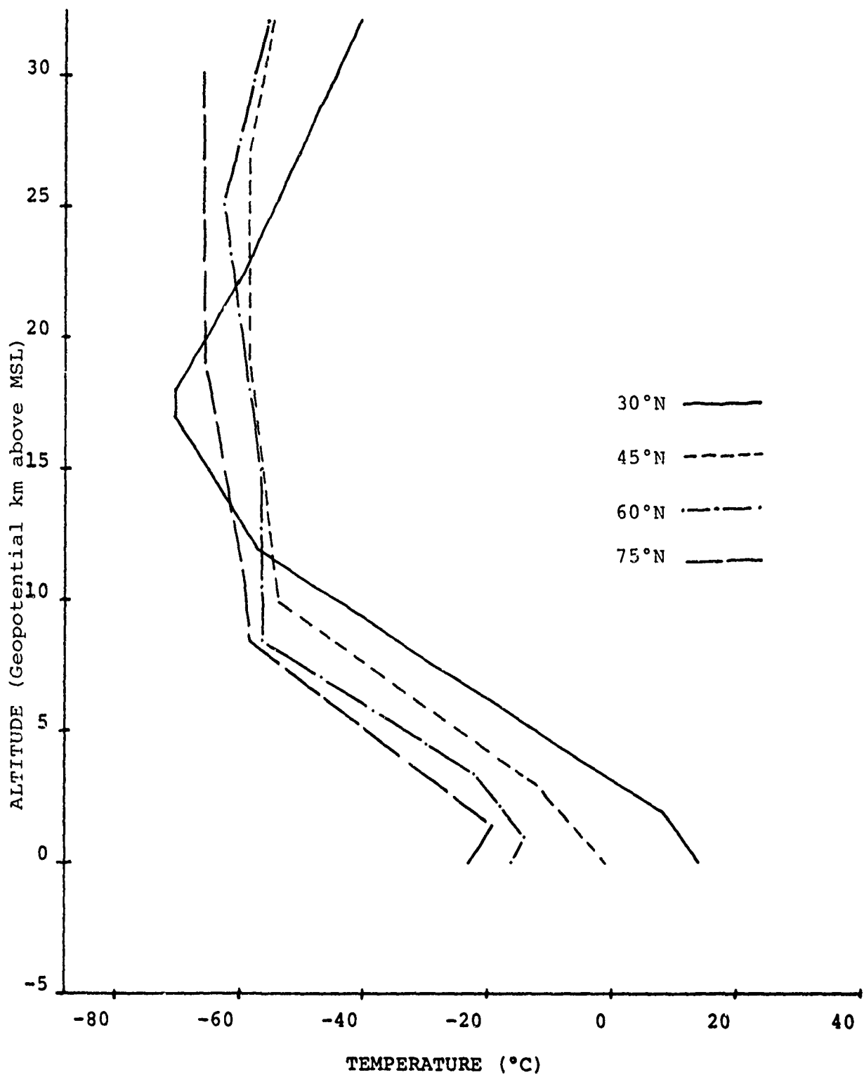
Figure 3. U.S. Standard Atmosphere Supplements, 1966 (January)
