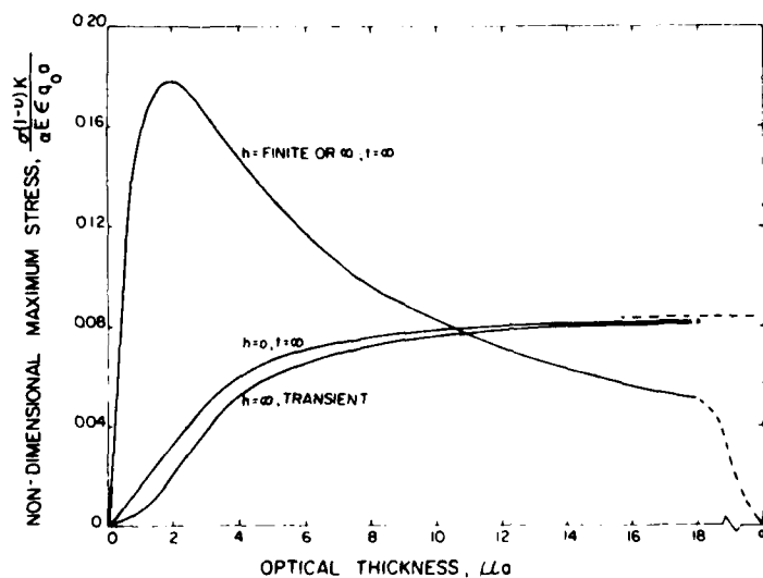
Fig. 2 Magnitude of maximum tensile thermal stresses as a function of optical thickness in flat plate assymmetrically heated by thermal radiation on one side and cooled by convection on the opposite side.
