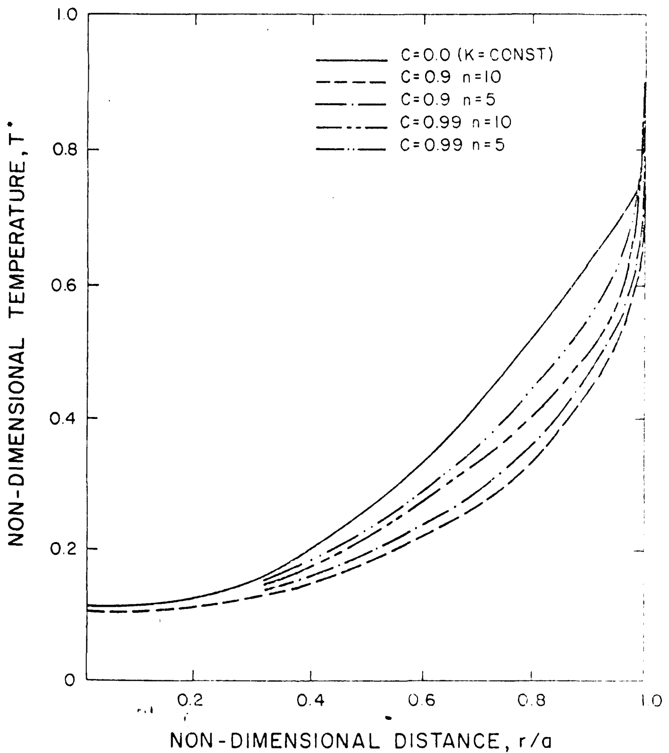
Fig. 2a. Transient temperature distributions in solid circular cylinders subjected to sudden convective heating at time of maximum tensile stress for the spatial distributions of the thermal conductivity given in fig. 2.
