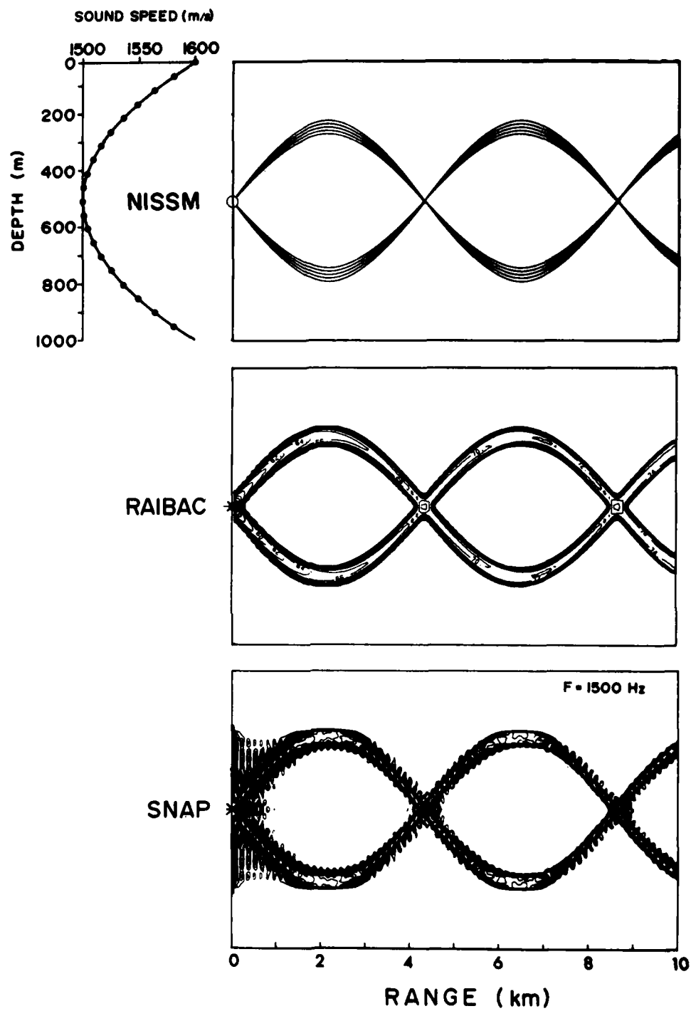
FIG. 3 INTER-MODEL COMPARISON FOR DEEP WATER ENVIRONMENT
