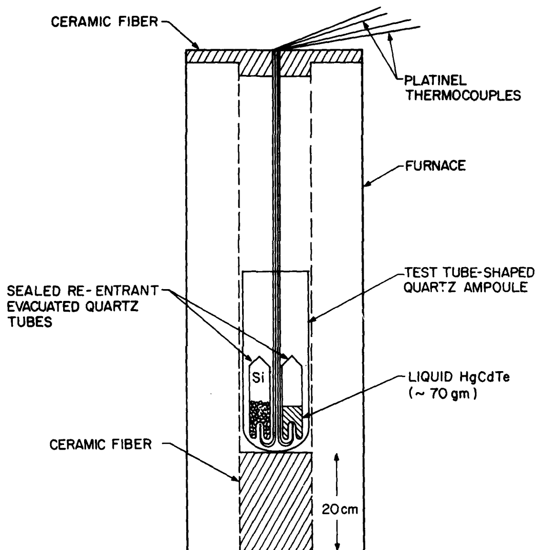
Fig. 1. A schematic of the differential thermal analysis (DTA) apparatus used to measure liquidus temperatures of the Te-rich HgCdTe phase diagram.
