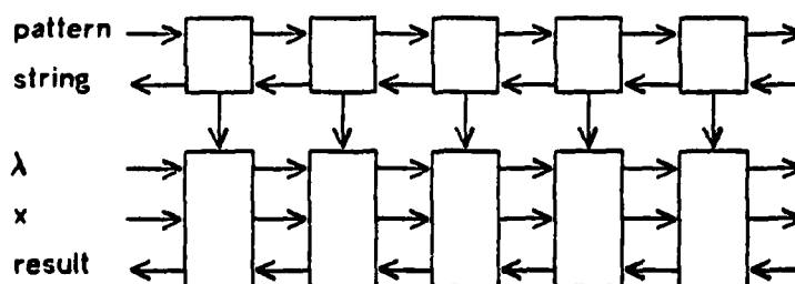
Figure 3-3: Comparators (on the top) and accumulators (on the bottom.)
