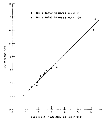
FIGURE 16. CORRELATION OF ASTM ACID NUMBER VS FIELD KIT ACID NUMBERS
