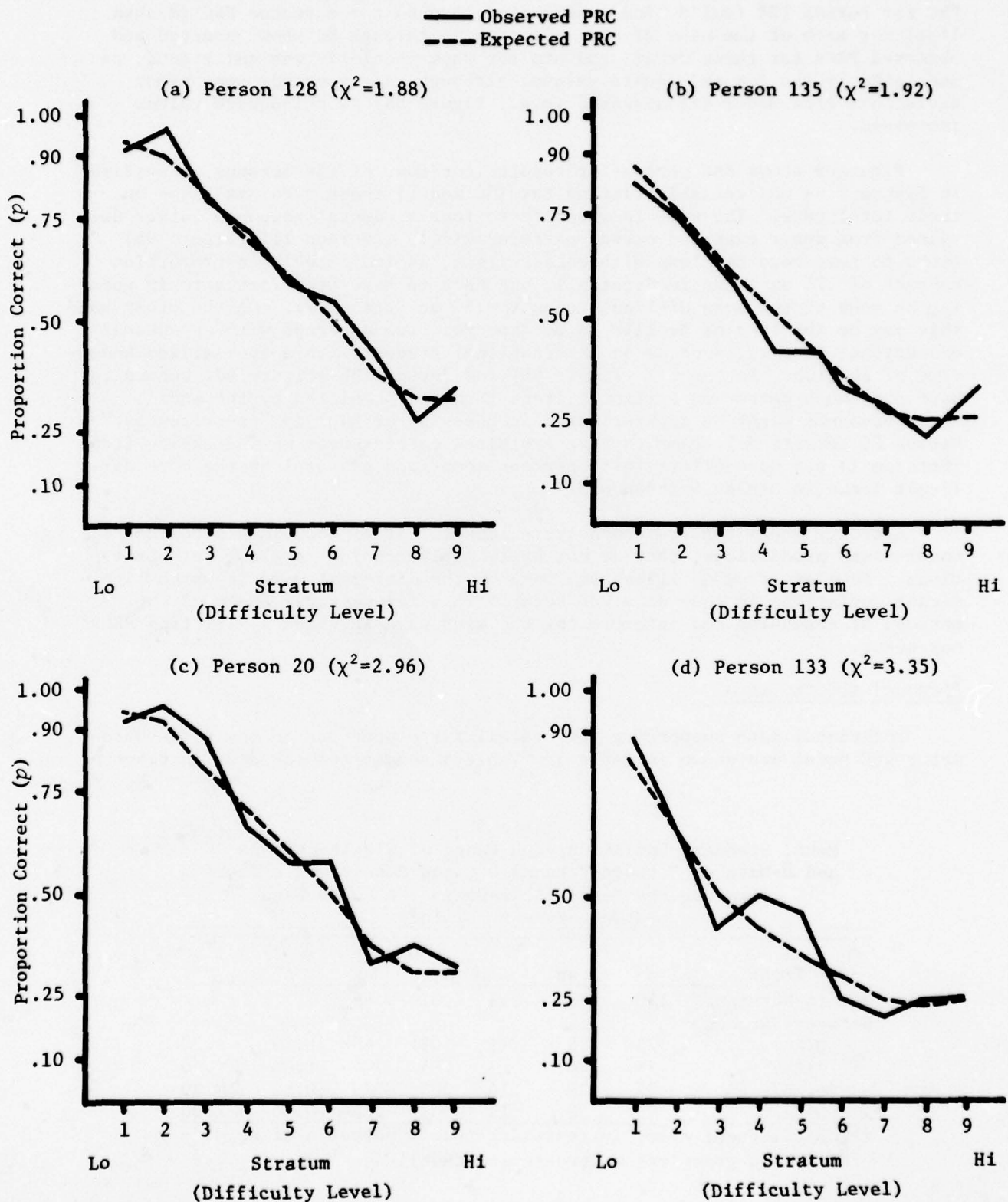
Figure 8 Observed and Expected Person Response Curves (PRCs) for Four Persons Whose Responses Reliably Fit the Three-Parameter ICC Model
