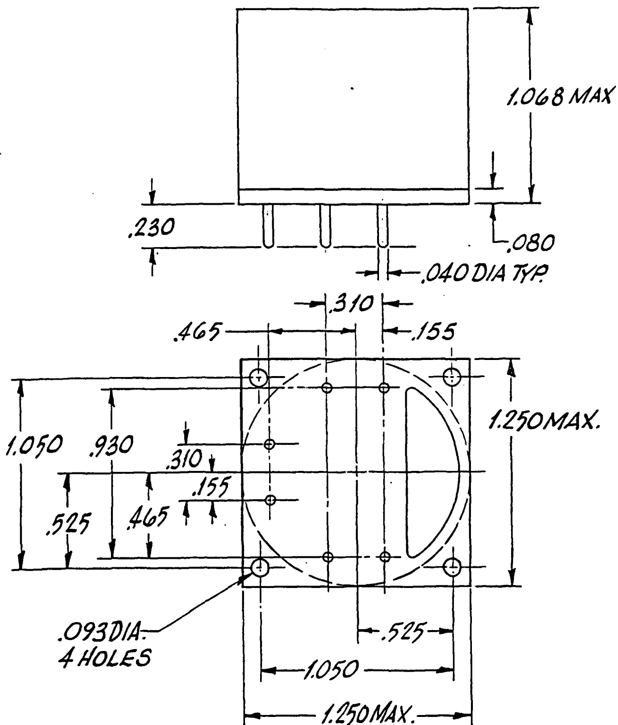
FIGURE 1-1. OUTLINE DRAWING
