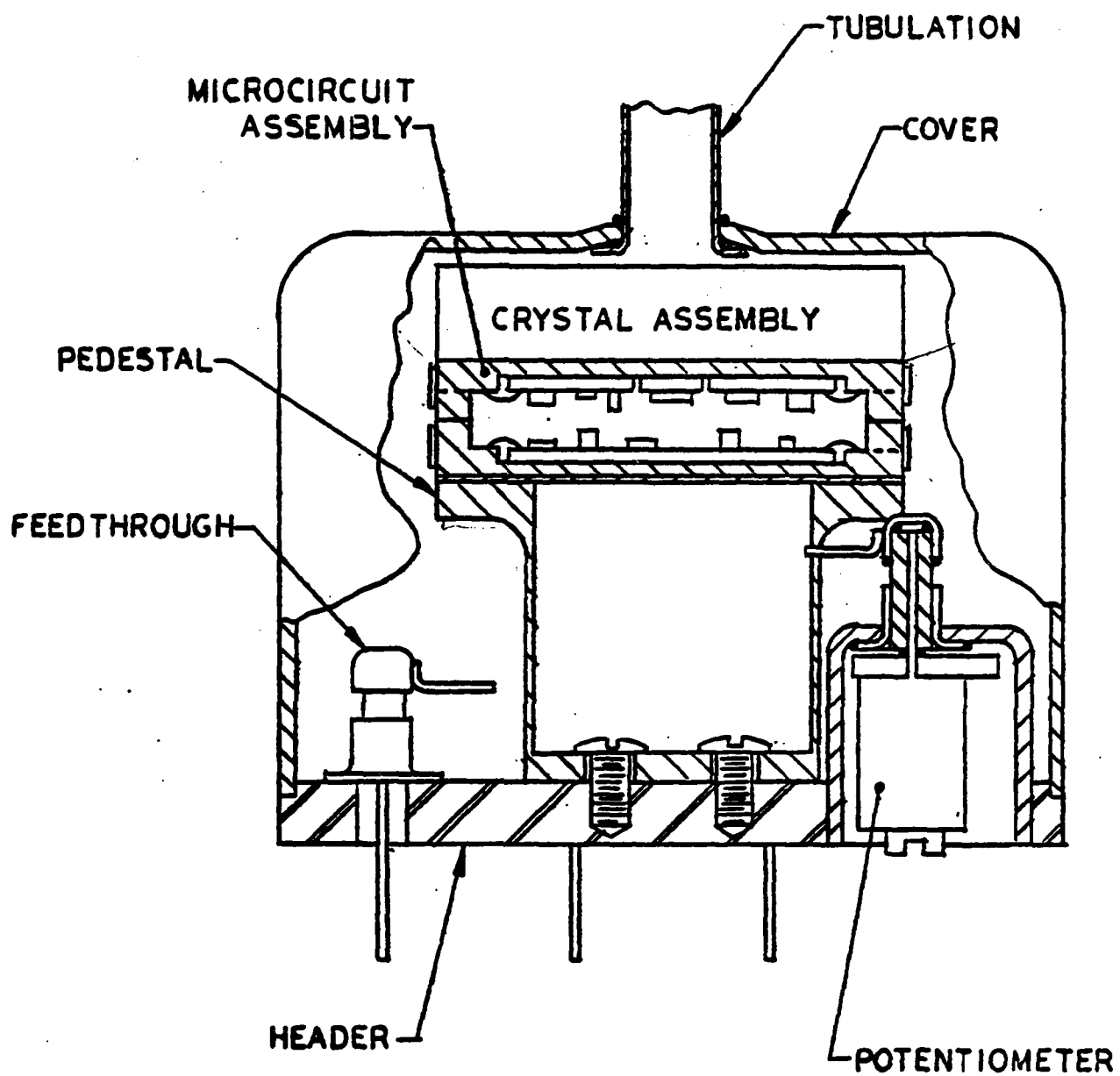
FIGURE 2-6 - OVERALL CONFIGURATION
