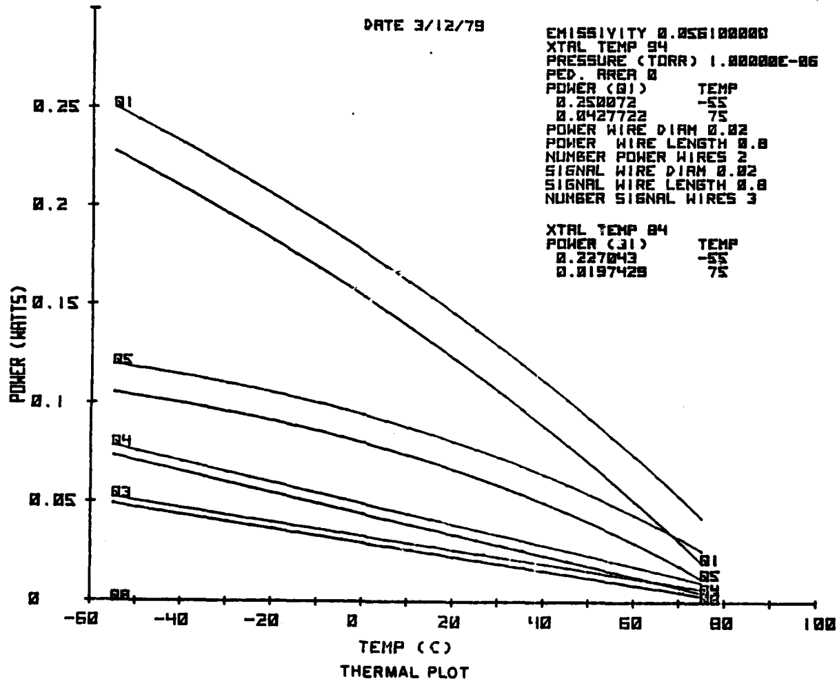
FIGURE 4-20. THERMAL PLOT
