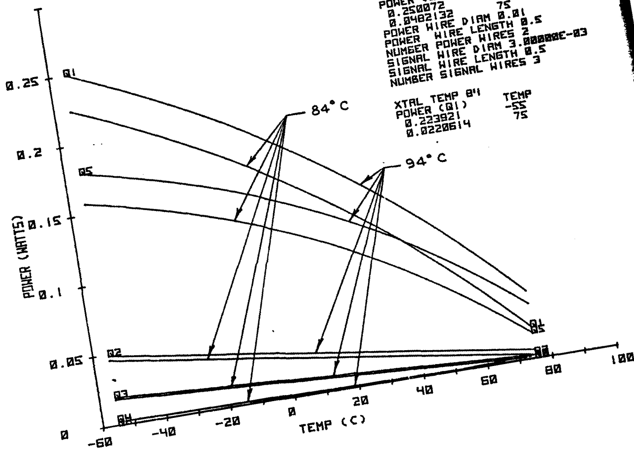
FIGURE 4-16. THERMAL PLOT
