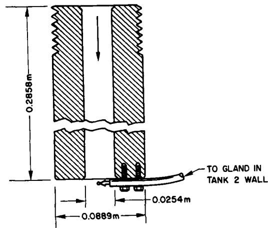
Fig. 4 - Sectional view of straight nozzle
