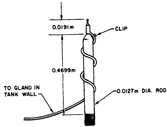
Fig. 3 - Thermocouple fixture
