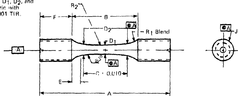
Figure 13. Fatigue specimen geometry.
