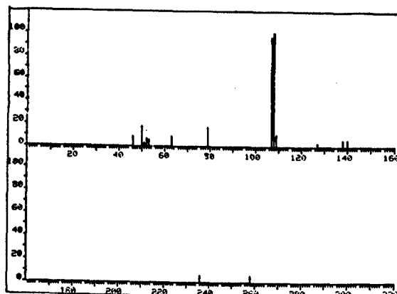
Figure 20. Mass spectrum of p-cresol.
