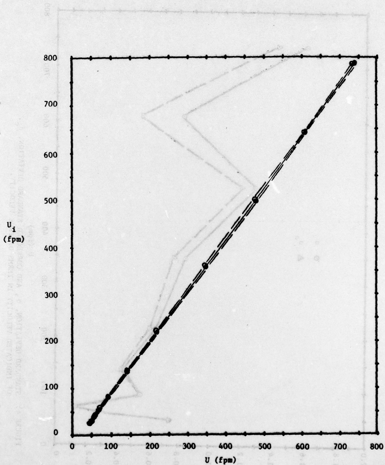
FIGURE 3. INDICATED VERSUS TRUE VELOCITY WITH \pm 2\sigma CURVES.
