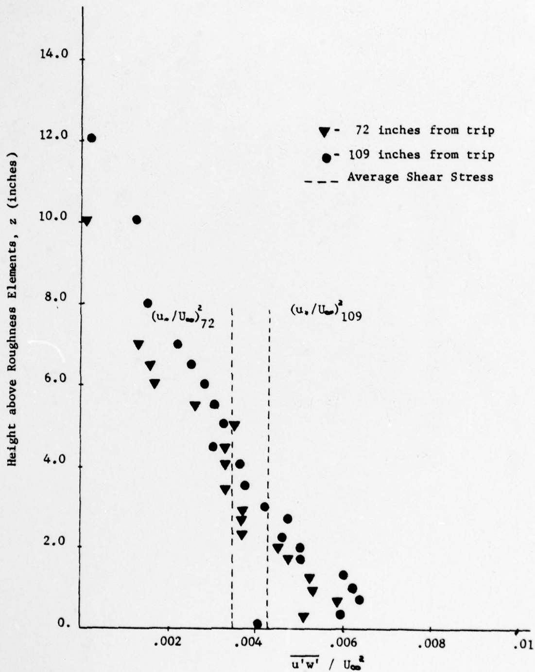
Figure 9 Vertical Distribution of Shear Stress at 72 and 109 inches Downwind
