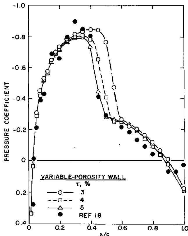
Figure 23. Model surface pressure distribution, M_\infty = 0.8 and \alpha = 0 deg.
