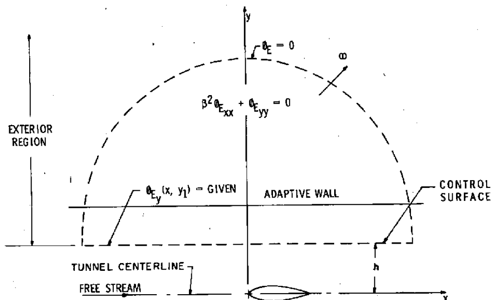
Figure 9. Boundary-value problem of exterior unconfined region.
