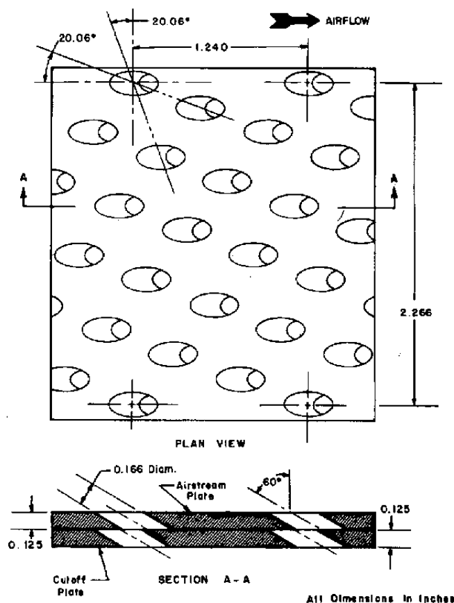
Figure 5. Variable-porosity wall.
