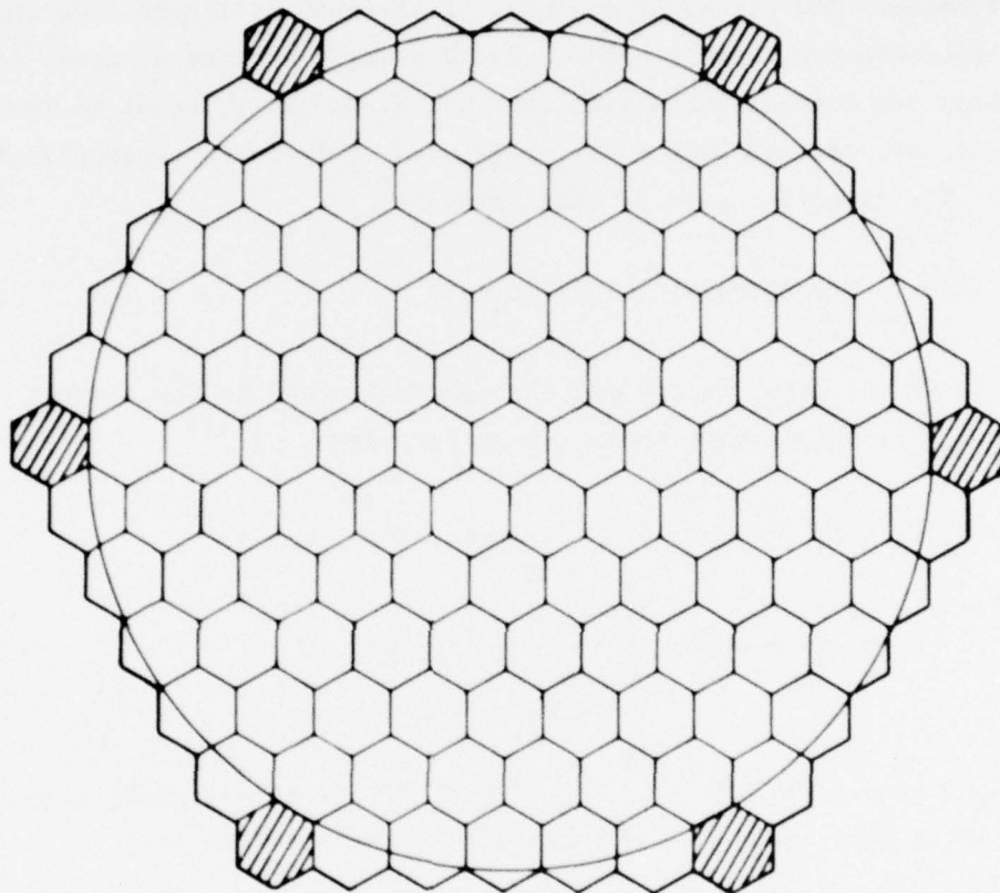
Fig. 2. 127-beam array.
