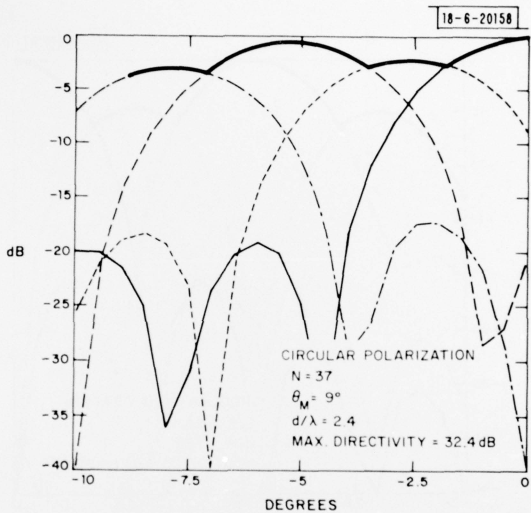
Fig. 9. Radiation patterns of 37-beam phased array antenna.
