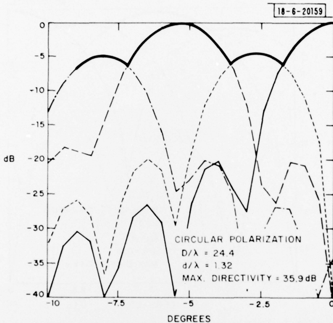
Fig. 10. Radiation patterns of 37-beam lens antenna.
