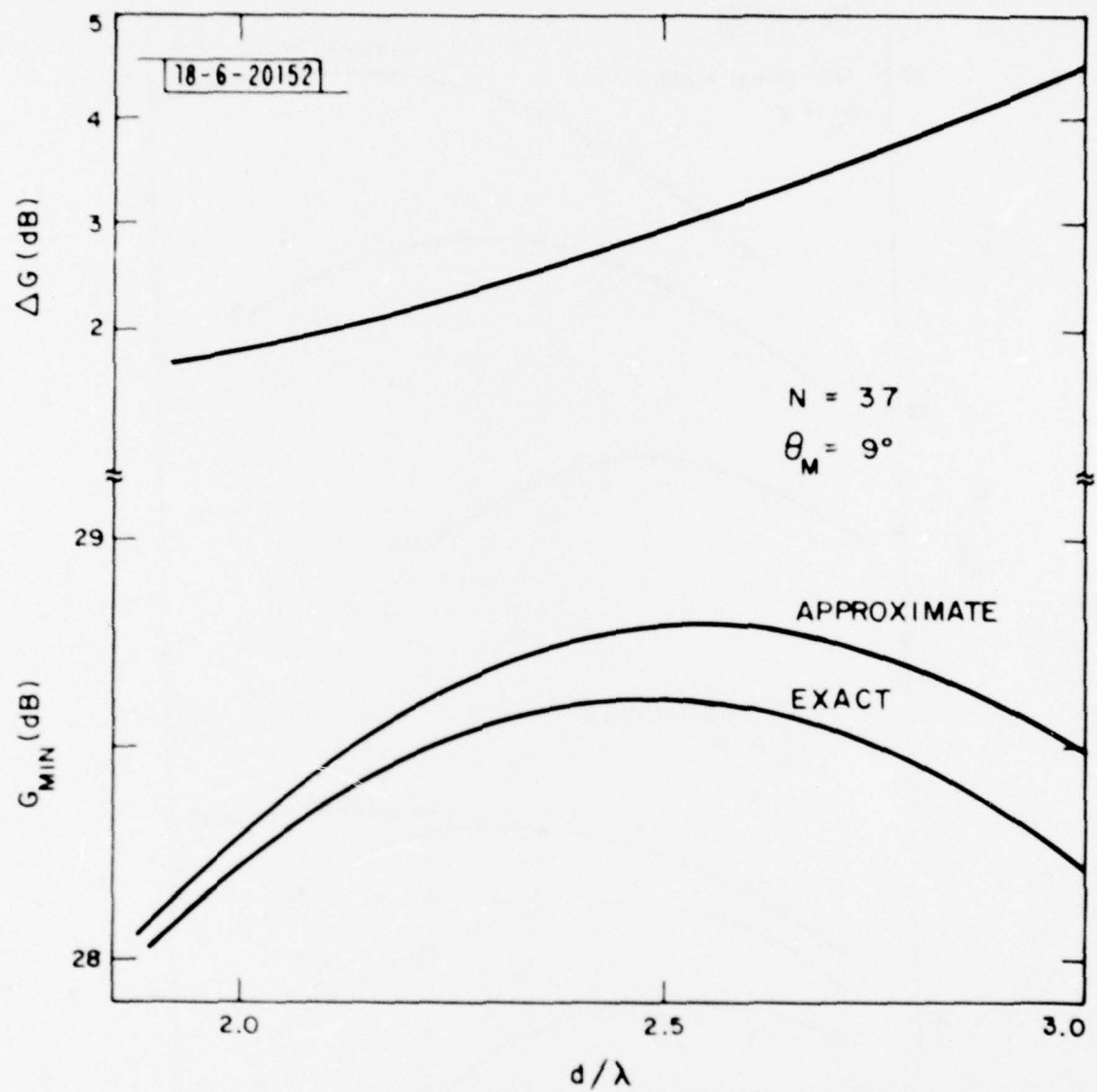
Fig.3. Minimum directive gain, G_{\text{MIN}} , and gain variation, \Delta G , of 37-beam phased array as a function of element diameter.
