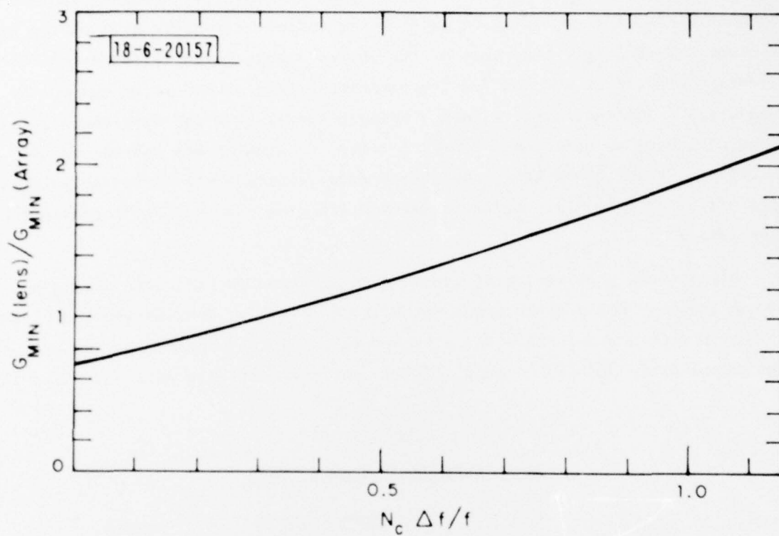
Fig. 8. Ratio of minimum directive gain of phased array and lens antennas.
