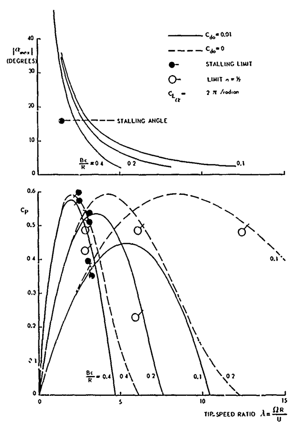
Fig. 4.33 Influence of rotor solidity Bc/R and profile drag C_{do} on C_p and |\alpha_{max}| of a two-dimensional vertical-axis turbine, according to a simplified theory
