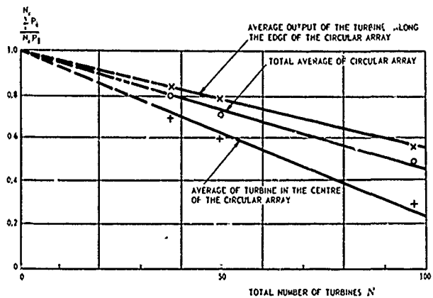
Fig. 5.34 Output averaged over the several wind directions in isotropic wind, according to Ref. 5.26
