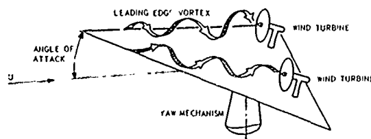
Fig. 3.17 Vortex augmentor concept of Ref. 3.18
