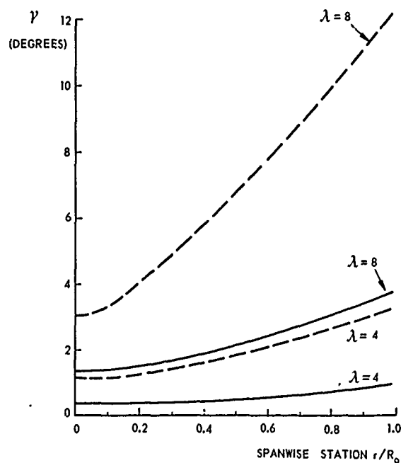
Fig. D.4 Deflection angle of the blade axis of an optimally operating horizontal-axis turbine with zero bending moments in the rotor blade. B = 2 , C_1 = 1.0
