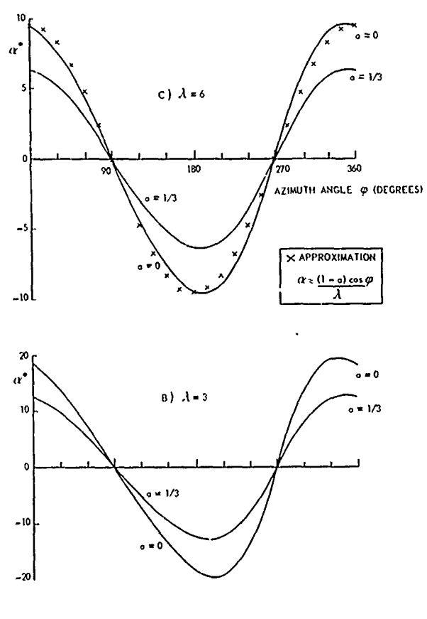
Fig. 4.31 Angle of attack as a function of the azimuth angle \varphi , the tip-speed ratio \lambda and induction factor a
