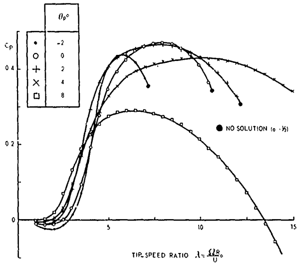
Fig. 4.24 Twisted blade design with linear taper B=2 , r_{hub}/R_0=0.10 Influence of blade pitch variation c/R_0 = 0.16 - 0.136 r/R_0 i = 11.380 (r/R_0) - 0.487 -15.0 (degrees) \theta_p blade pitch angle positive in the same direction as i . The pitch angle is defined as a rigid body rotation with respect to the blade twist distribution i=f(r/R_0)
