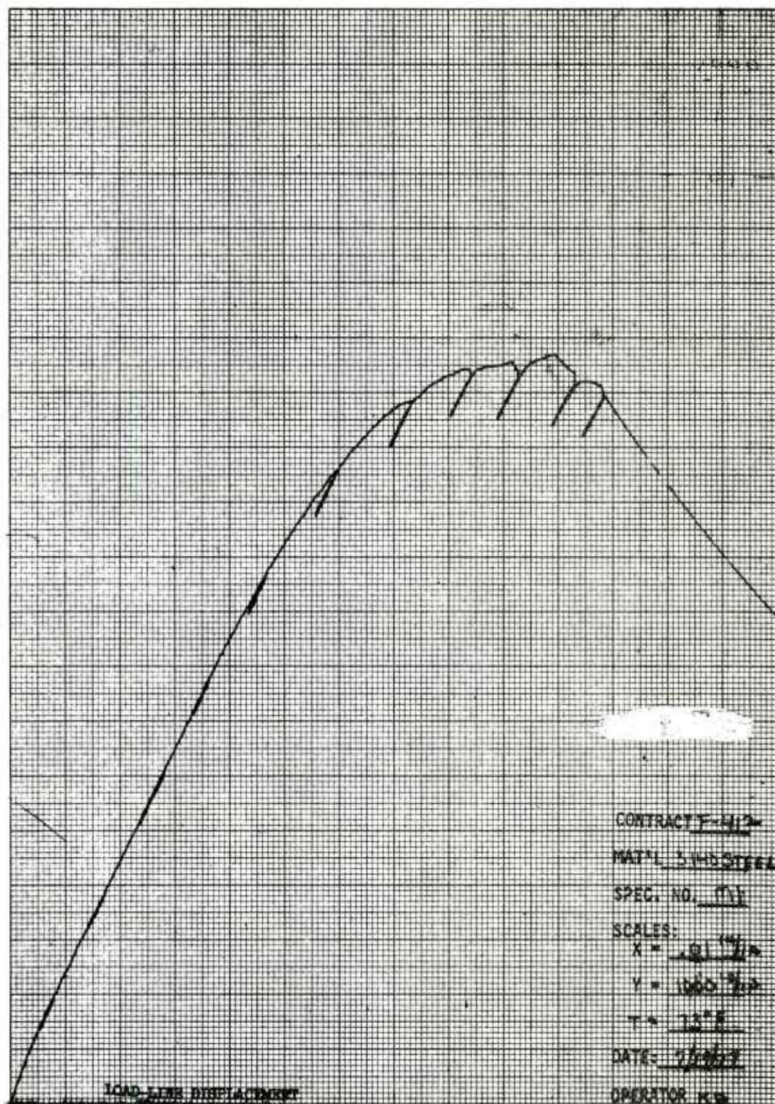
Figure 1. Load-line displacement curve of specimen M1.
