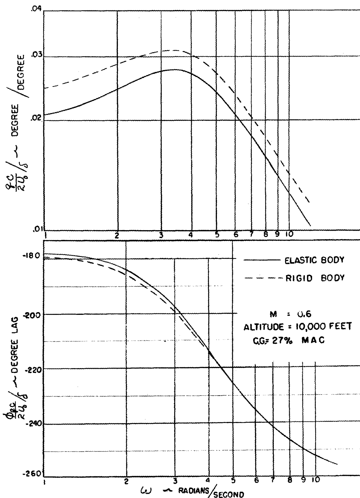
F-80A DYNAMIC RESPONSE CURVES PITCHING VELOCITY AMPLITUDE AND PHASE VS. FREQUENCY
