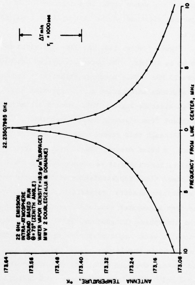
Figure 4. Emission spectra (Longbothum, 1977)
