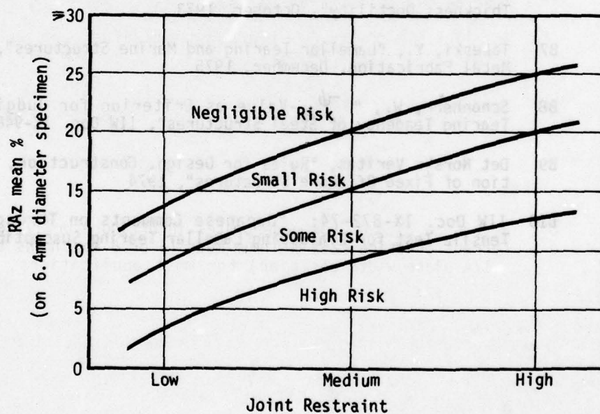
Fig B-3 Approximate Risk of Lamellar Tearing for C and C-Mn Steels. Specified minimum yield stress < 40.8 kg/mm 2
