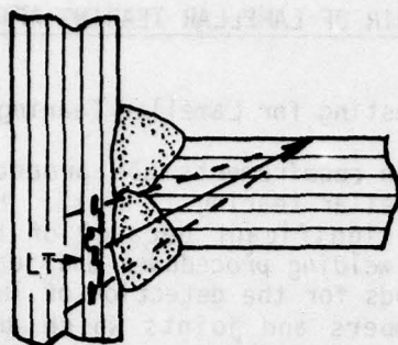
Shear or Angle Probe
