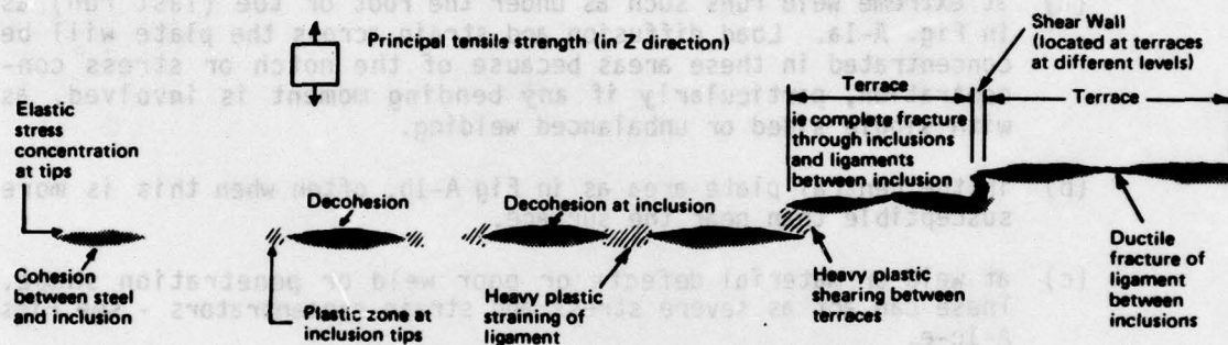
Fig 10 Mechanism of LT.
