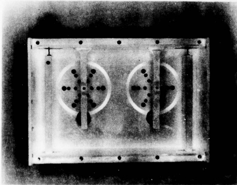
Figure 6.12 Small Comb Line Filter
