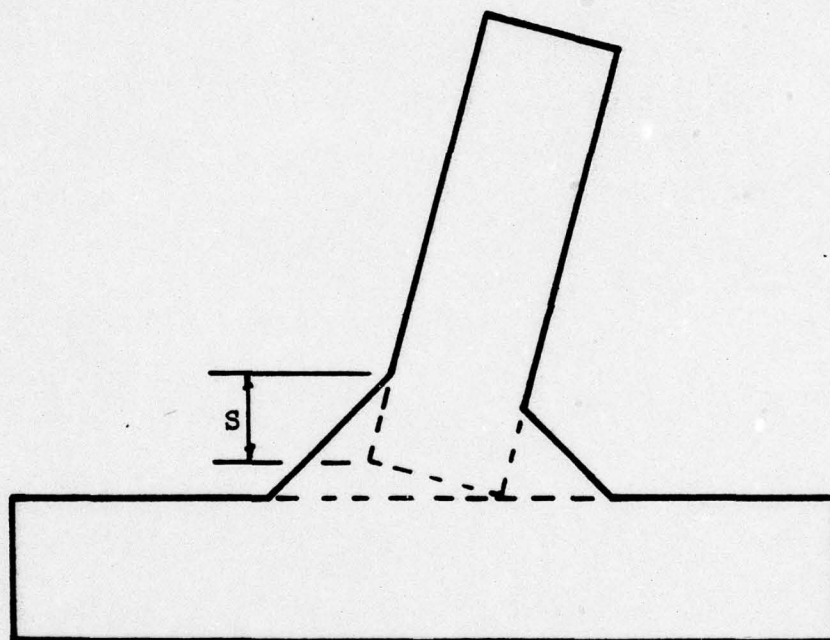
FIGURE 6.5. A SKEWED FILLET WELDED TEE JOINT
