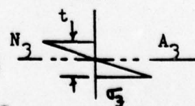
PLATE BENDING
