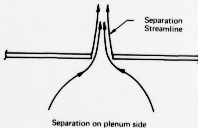
FIG. 3(b) SLOT FLOW MODELS
