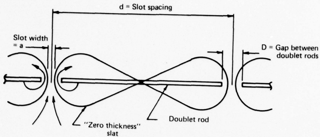
(a) Chen and Mears model of slat
