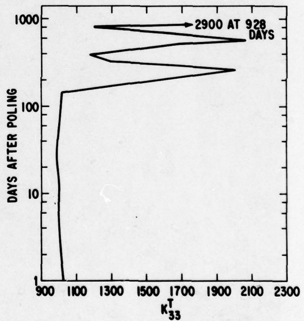
Fig. 6 Aging of the dielectric constant of a specimen of composition Pb(Zr_{.52}Tr_{.48})_{.97}Fe_{.01}Cr_{.02}O_3 .
