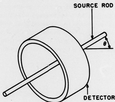
Figure 2. "Collimator" Code Geometry for Single Rod Spectrum. The monte carlo code "collimator" counts the photons (and their energy) which leave the rod, traverse the empty space, and enter the detector. Photons leaving the rod nearly parallel to the rod do not enter the detector and are therefore not counted
