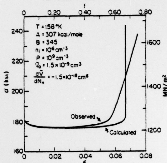
Fig. 4. Comparison of calculated and observed [1] true \sigma - \epsilon curves for TRIP steel of Fig. 1.
