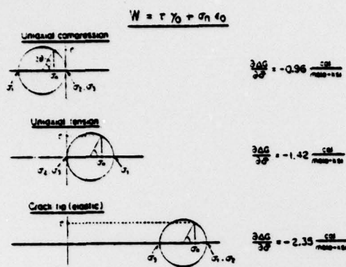
Fig. 5. Calculated work of resolved shear stress, \tau , and normal stress, \sigma_n , assisting transformation shape change with shear and normal strains, \gamma_0 and \epsilon_0 .
