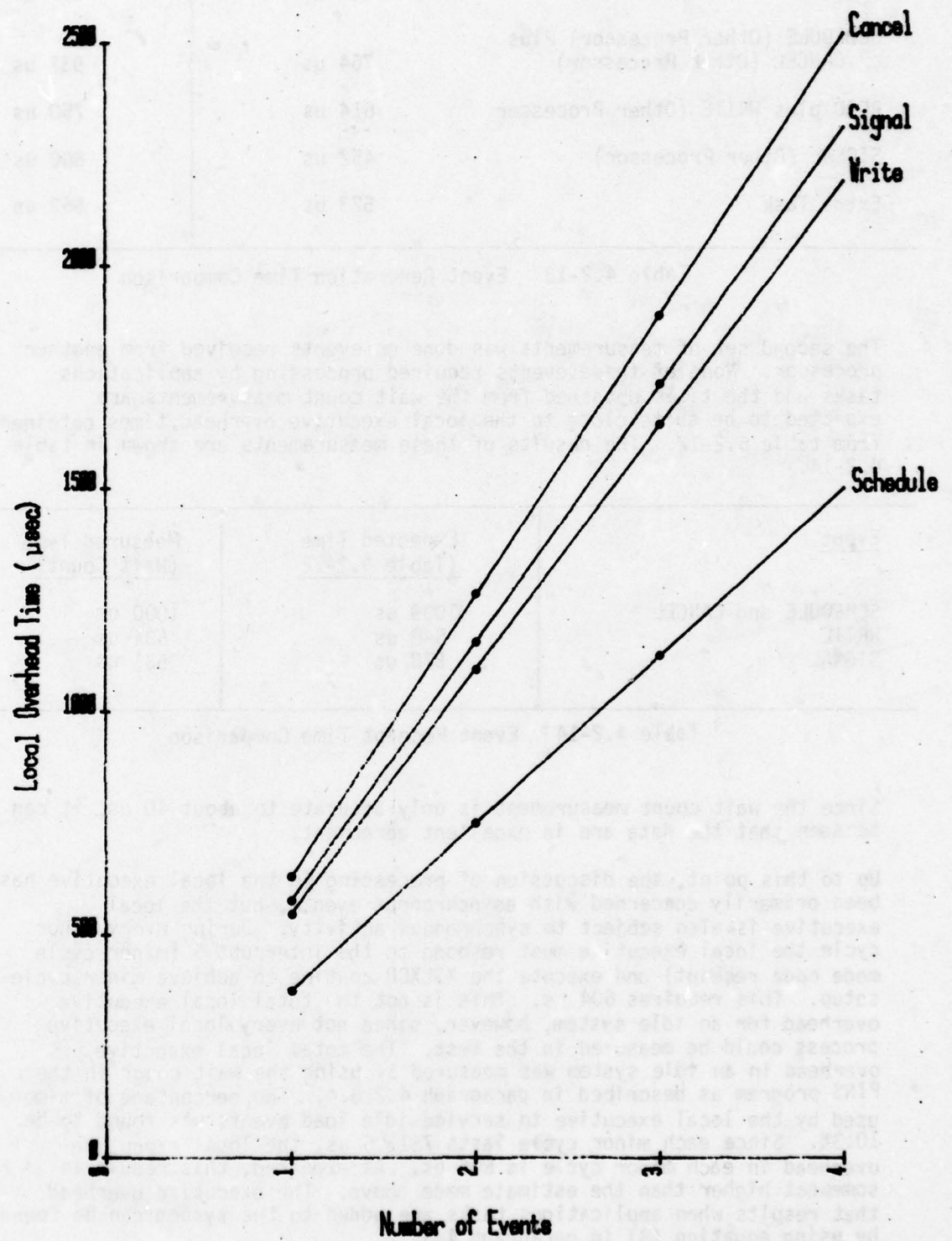
Figure 4.2-12 Local Executive Service Times - Received From Other Processor
