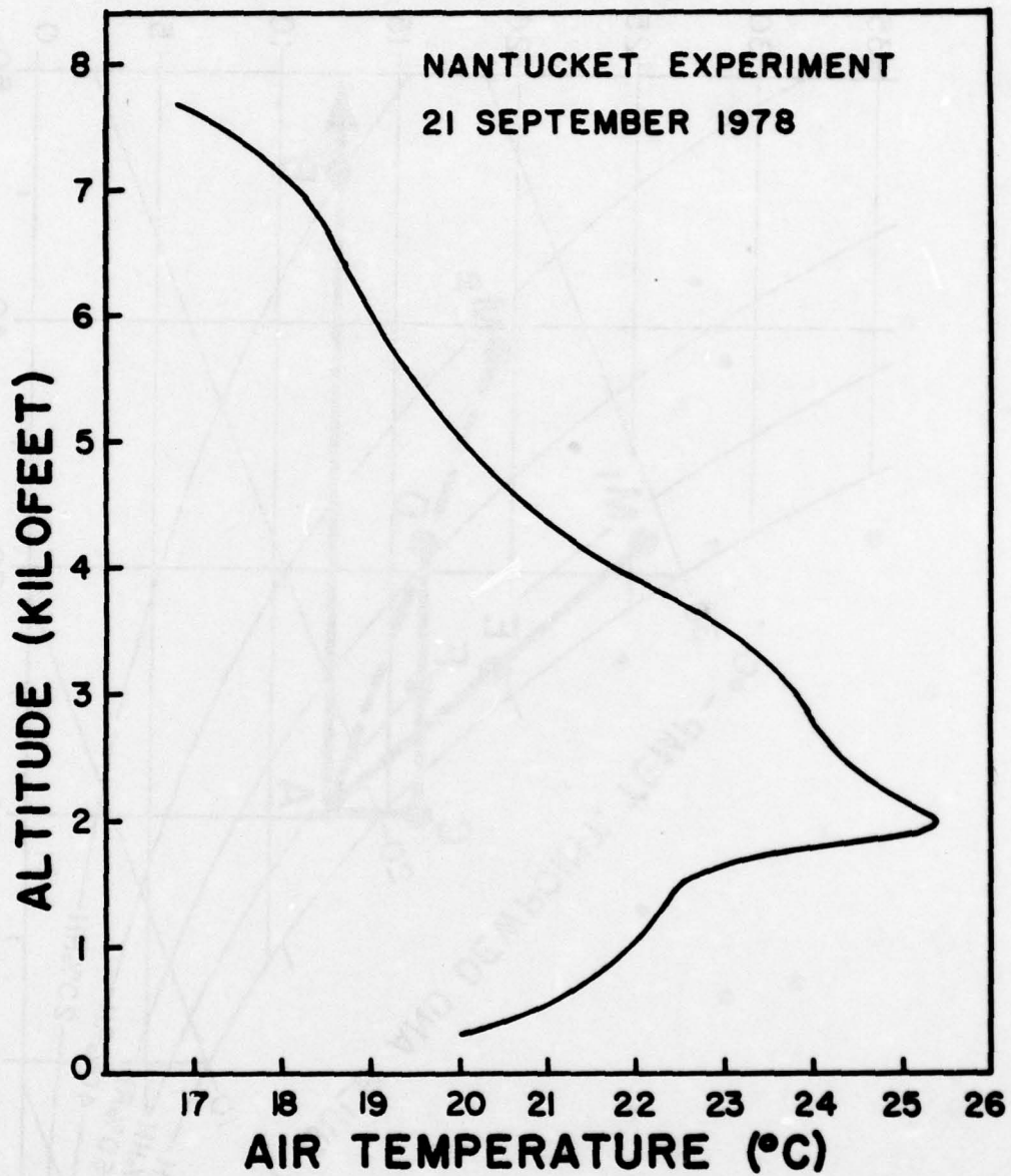
Fig. 7 — Temperature profile
