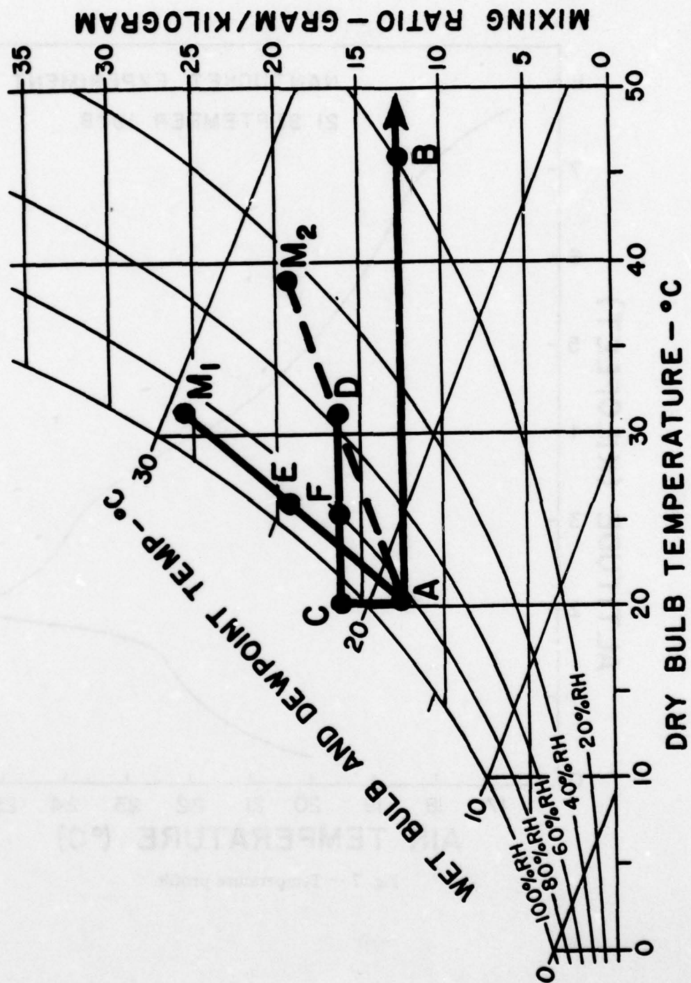
Fig. 6 — Thermodynamic processes
