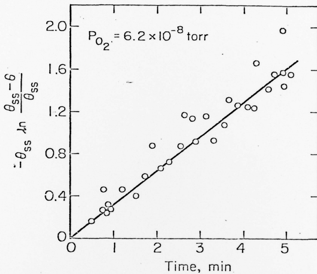
Figure 4. Surface coverage of oxygen as a linearized function of time.
