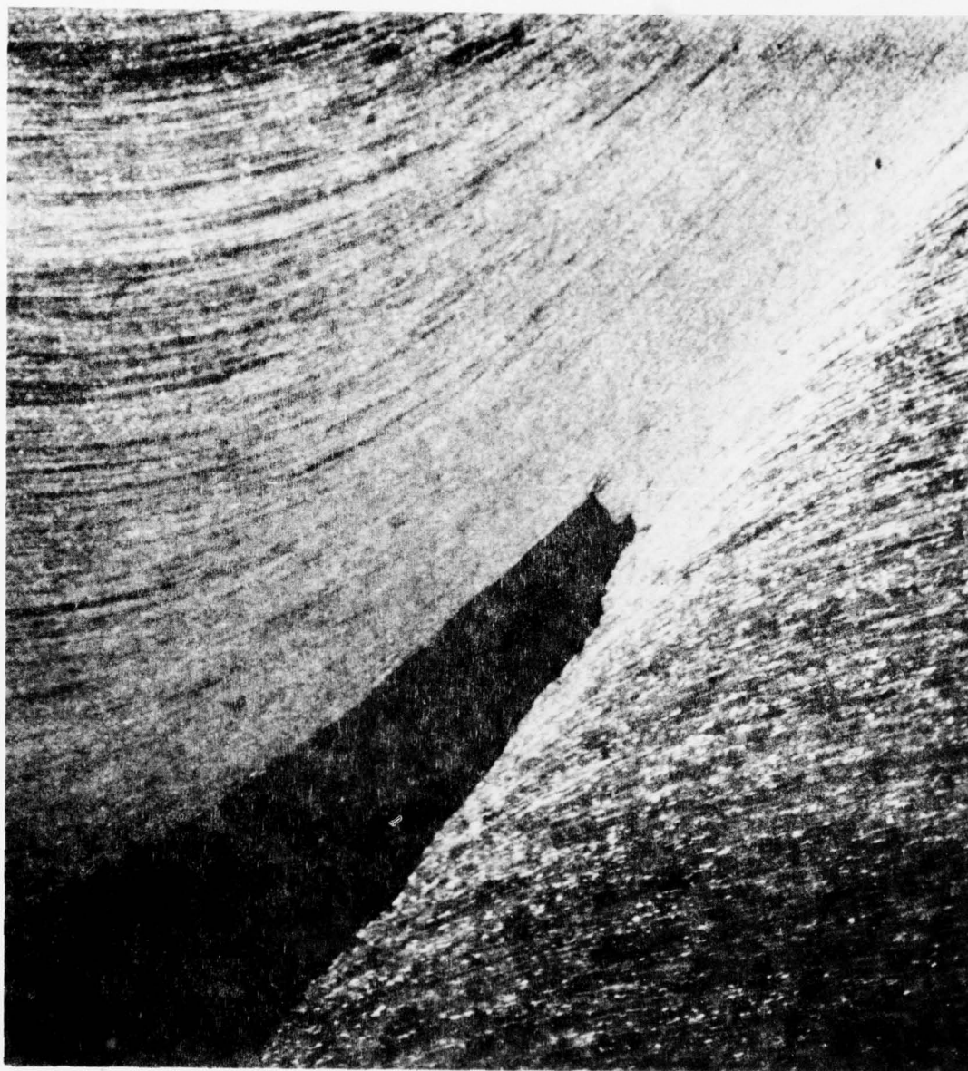
Fig. 7. Crack tip as central burst approaches complete development.
