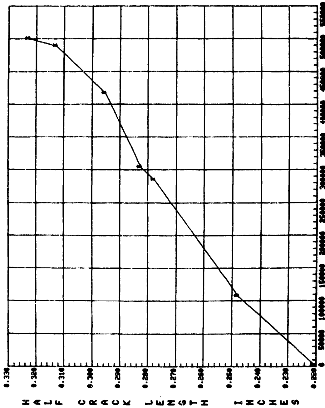
TEST LIFE N (CYCLES) Figure 94. Crack growth curve for test M-74.
