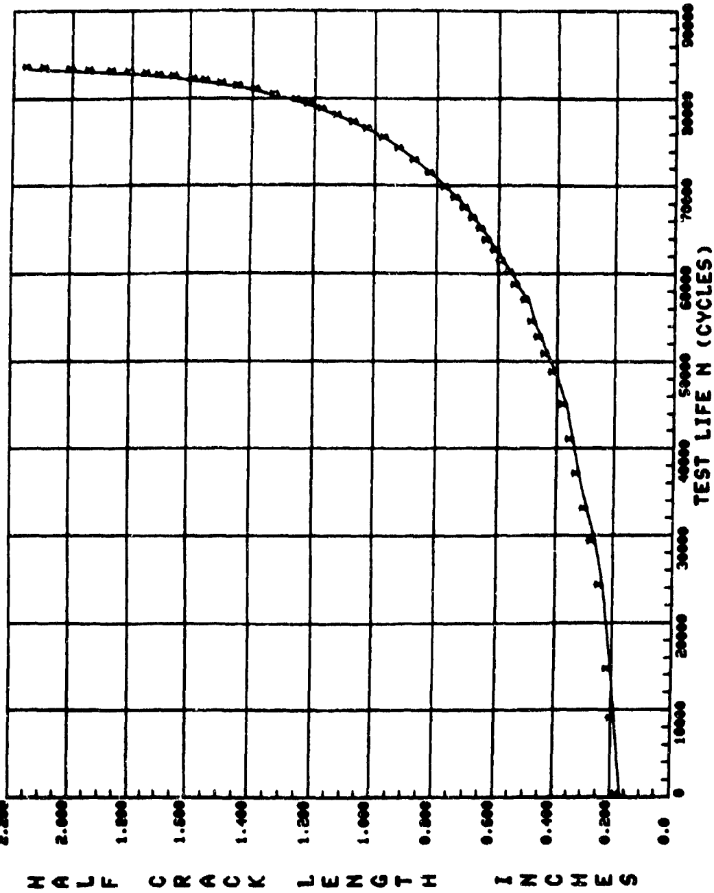
Figure 92. Crack growth curve for test M-72A.
